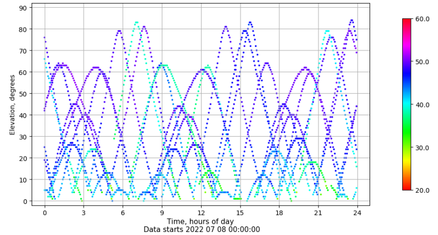
Time-elevation plot for station GIRO. Signal to Noise S1C Data file GIRO00ESP_R_2022189.xtr
