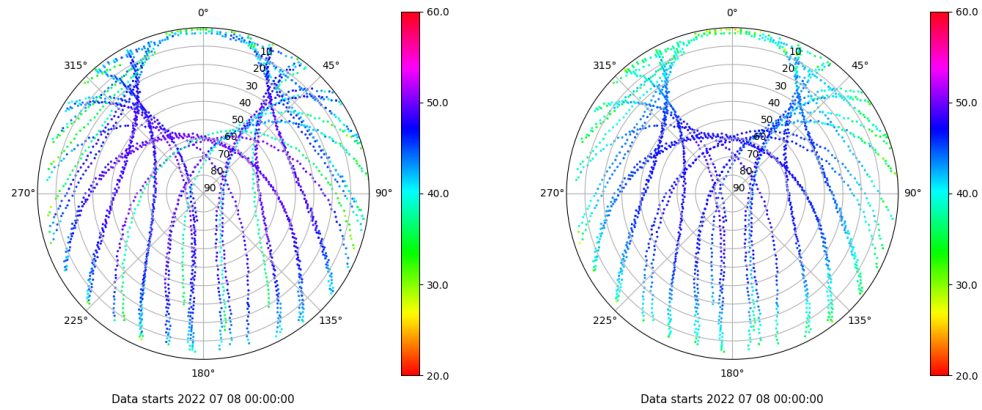
Skyplot for station GIRO. Signal to Noise S1C Data file GIRO00ESP_R_2022189.xtr Skyplot for station GIRO. Signal to Noise S2P Data file GIRO00ESP_R_2022189.xtr
