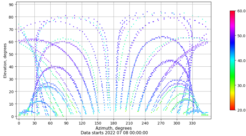
Azimuth-elevation plot for station GIRO. Signal to Noise S1C Data file GIRO00ESP_R_2022189.xtr
