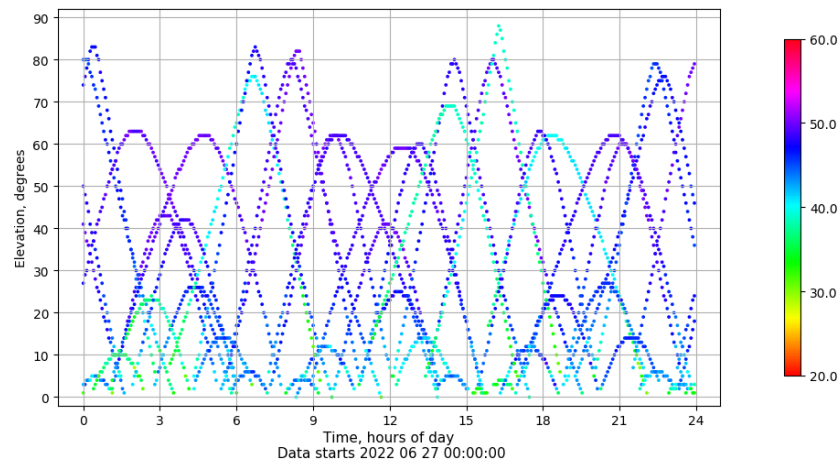
Time-elevation plot for station GIRO. Signal to Noise S1C Data file GIRO00ESP_R_2022178.xtr
