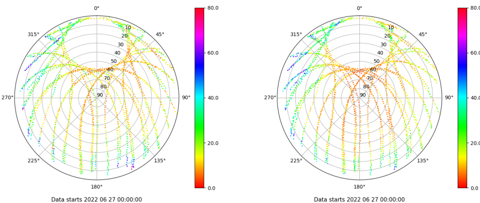
Skyplot for station GIRO. Parameter M1C Data file GIRO00ESP_R_2022178.xtr Skyplot for station GIRO. Parameter M2P Data file GIRO00ESP_R_2022178.xtr
