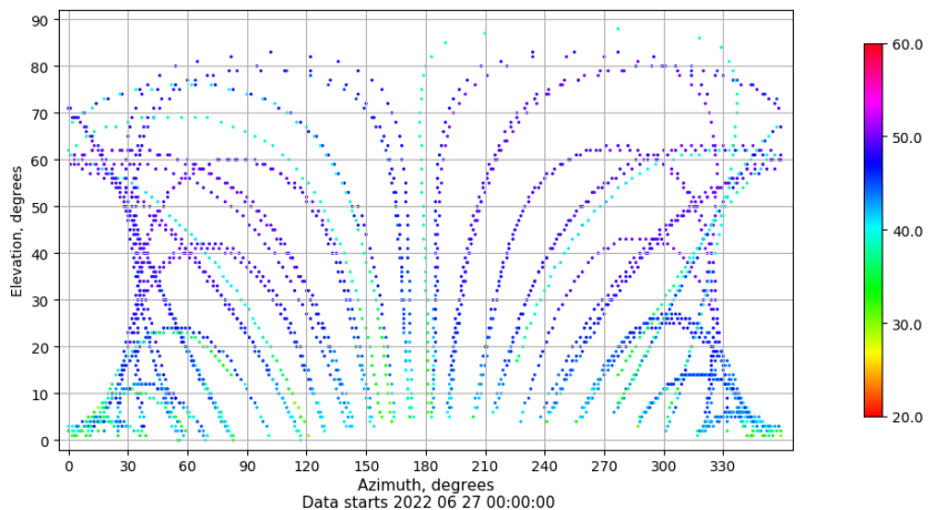
Azimuth-elevation plot for station GIRO. Signal to Noise S1C Data file GIRO00ESP_R_2022178.xtr
