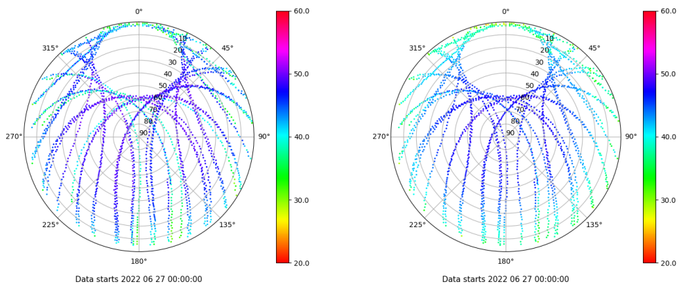
Skyplot for station GIRO. Signal to Noise S1C Data file GIRO00ESP_R_2022178.xtr Skyplot for station GIRO. Signal to Noise S2P Data file GIRO00ESP_R_2022178.xtr
