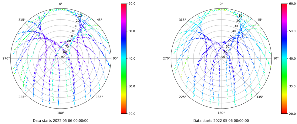
Skyplot for station GIRO. Signal to Noise S1C Data file GIRO00ESP_R_2022126.xtr Skyplot for station GIRO. Signal to Noise S2P Data file GIRO00ESP_R_2022126.xtr
