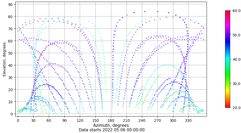
Azimuth-elevation plot for station GIRO. Signal to Noise S1C Data file GIRO00ESP_R_2022126.xtr
