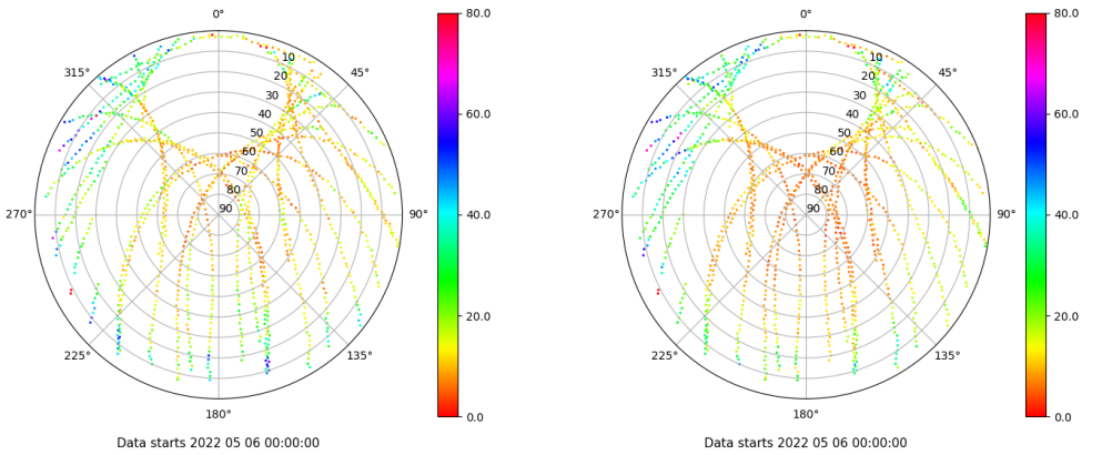
Skyplot for station GIRO. Parameter M1C Data file GIRO00ESP_R_2022126.xtr Skyplot for station GIRO. Parameter M2P Data file GIRO00ESP_R_2022126.xtr
