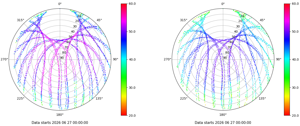
Skyplot for station EIVI. Signal to Noise S1C Data file EIVI00ESP_R_2026178.xtr Skyplot for station EIVI. Signal to Noise S2P Data file EIVI00ESP_R_2026178.xtr
