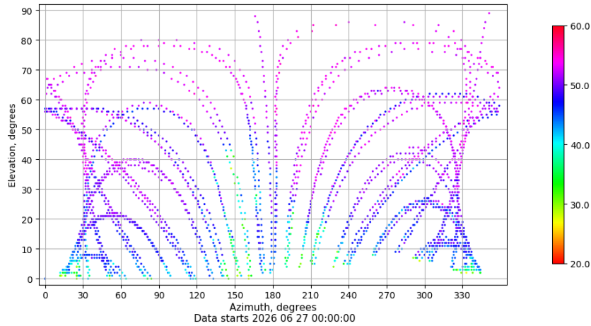
Azimuth-elevation plot for station EIVI. Signal to Noise S1C Data file EIVI00ESP_R_2026178.xtr
