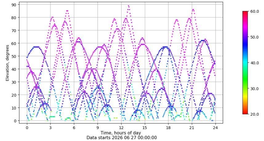
Time-elevation plot for station EIVI. Signal to Noise S1C Data file EIVI00ESP_R_2026178.xtr
