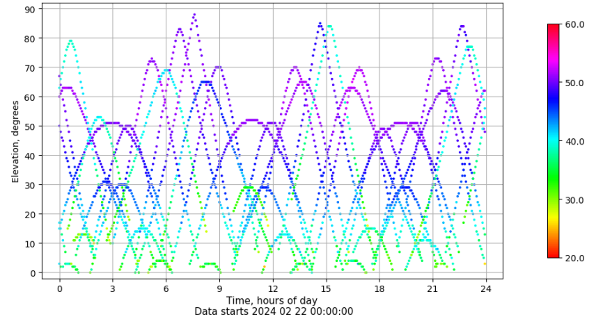
Time-elevation plot for station CEU1. Signal to Noise S1C Data file CEU100ESP_R_2024053.xtr
