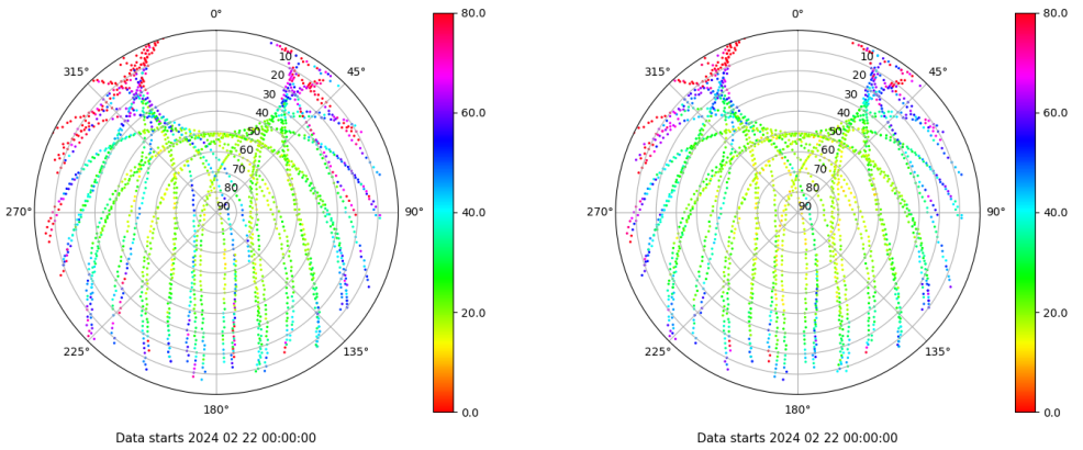
Skyplot for station CEU1. Parameter M1C Data file CEU100ESP_R_2024053.xtr Skyplot for station CEU1. Parameter M2C Data file CEU100ESP_R_2024053.xtr
