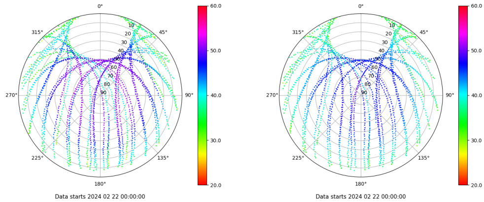
Skyplot for station CEU1. Signal to Noise S1C Data file CEU100ESP_R_2024053.xtr Skyplot for station CEU1. Signal to Noise S2C Data file CEU100ESP_R_2024053.xtr
