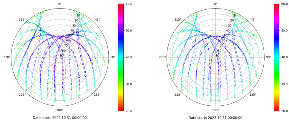
Skyplot for station CEU1. Signal to Noise S1C Data file CEU100ESP_R_2022304.xtr Skyplot for station CEU1. Signal to Noise S2C Data file CEU100ESP_R_2022304.xtr
