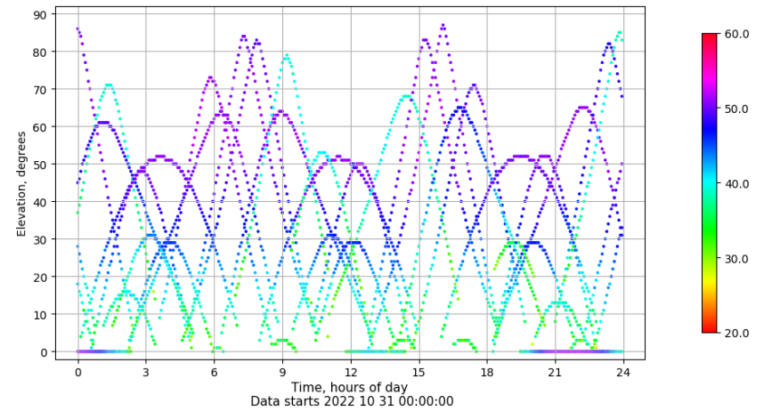
Time-elevation plot for station CEU1. Signal to Noise S1C Data file CEU100ESP_R_2022304.xtr
