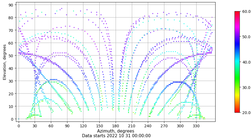
Azimuth-elevation plot for station CEU1. Signal to Noise S1C Data file CEU100ESP_R_2022304.xtr
