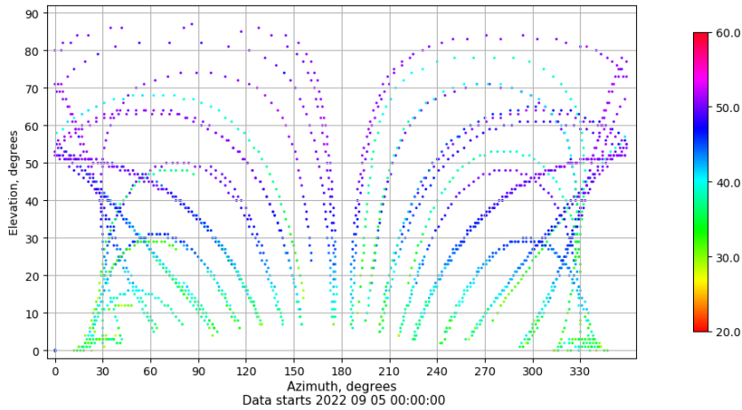
Azimuth-elevation plot for station CEU1. Signal to Noise S1C Data file CEU100ESP_R_2022248.xtr
