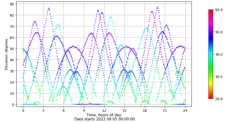
Time-elevation plot for station CEU1. Signal to Noise S1C Data file CEU100ESP_R_2022248.xtr
