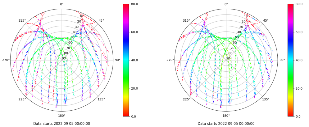
Skyplot for station CEU1. Parameter M1C Data file CEU100ESP_R_2022248.xtr Skyplot for station CEU1. Parameter M2C Data file CEU100ESP_R_2022248.xtr
