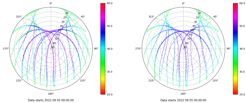
Skyplot for station CEU1. Signal to Noise S1C Data file CEU100ESP_R_2022248.xtr Skyplot for station CEU1. Signal to Noise S2C Data file CEU100ESP_R_2022248.xtr
