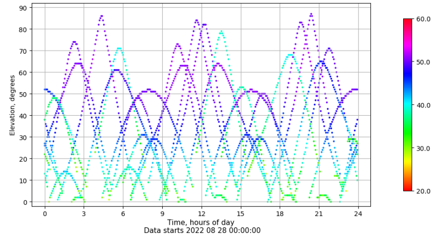
Time-elevation plot for station CEU1. Signal to Noise S1C Data file CEU100ESP_R_2022240.xtr
