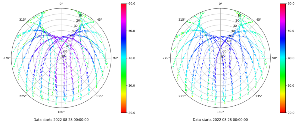
Skyplot for station CEU1. Signal to Noise S1C Data file CEU100ESP_R_2022240.xtr Skyplot for station CEU1. Signal to Noise S2C Data file CEU100ESP_R_2022240.xtr
