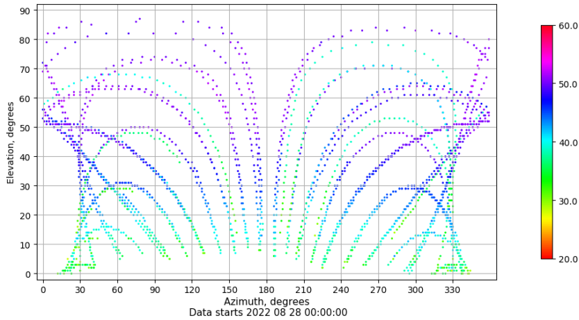
Azimuth-elevation plot for station CEU1. Signal to Noise S1C Data file CEU100ESP_R_2022240.xtr
