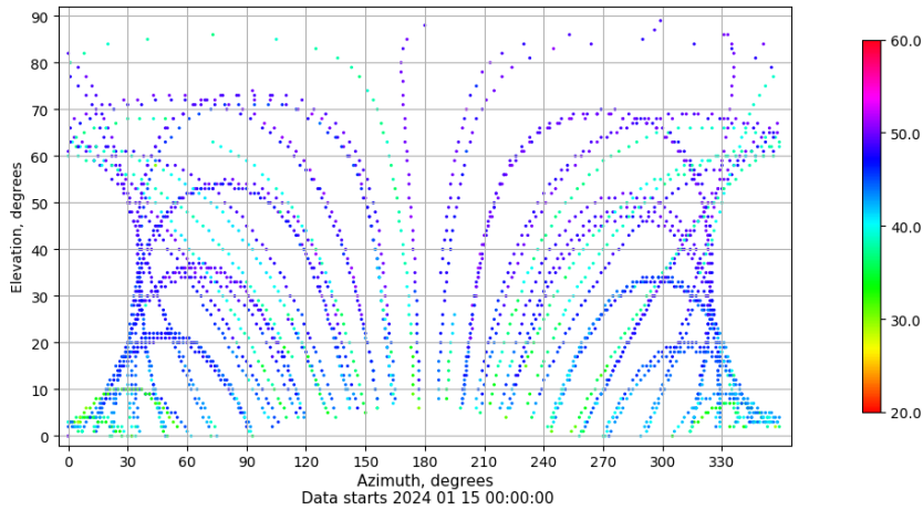
Azimuth-elevation plot for station CANT. Signal to Noise S1C Data file CANT00ESP_R_2024015.xtr
