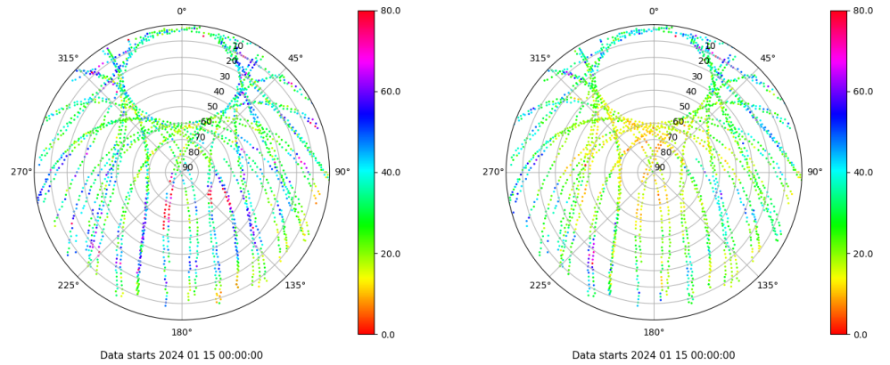
Skyplot for station CANT. Parameter M1C Data file CANT00ESP_R_2024015.xtr Skyplot for station CANT. Parameter M2P Data file CANT00ESP_R_2024015.xtr
