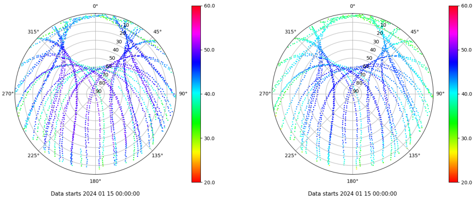
Skyplot for station CANT. Signal to Noise S1C Data file CANT00ESP_R_2024015.xtr Skyplot for station CANT. Signal to Noise S2P Data file CANT00ESP_R_2024015.xtr
