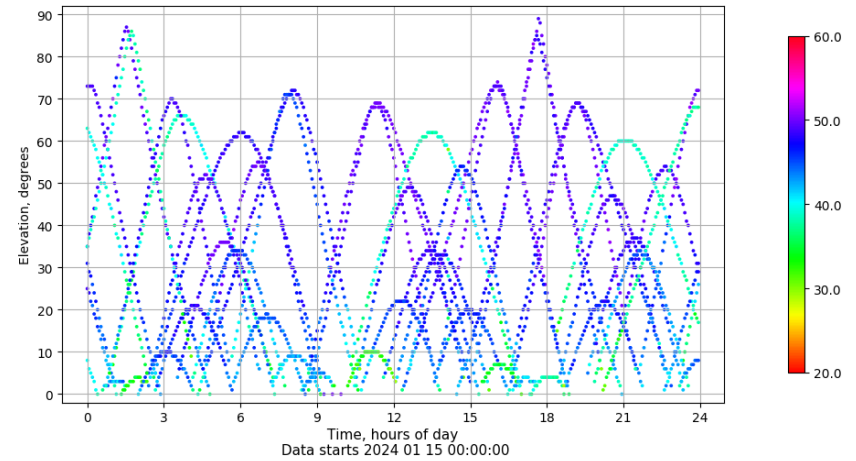
Time-elevation plot for station CANT. Signal to Noise S1C Data file CANT00ESP_R_2024015.xtr
