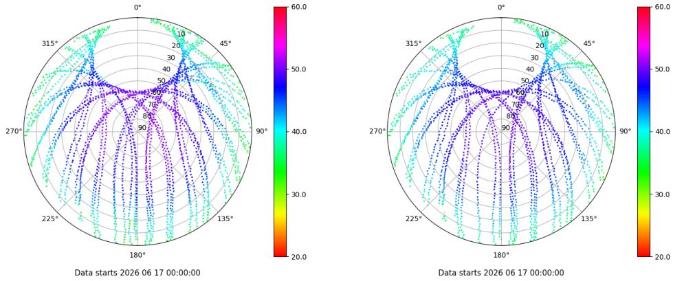
Skyplot for station BCL1. Signal to Noise S1C Data file BCL100ESP_R_2026168.xtr Skyplot for station BCL1. Signal to Noise S2P Data file BCL100ESP_R_2026168.xtr
