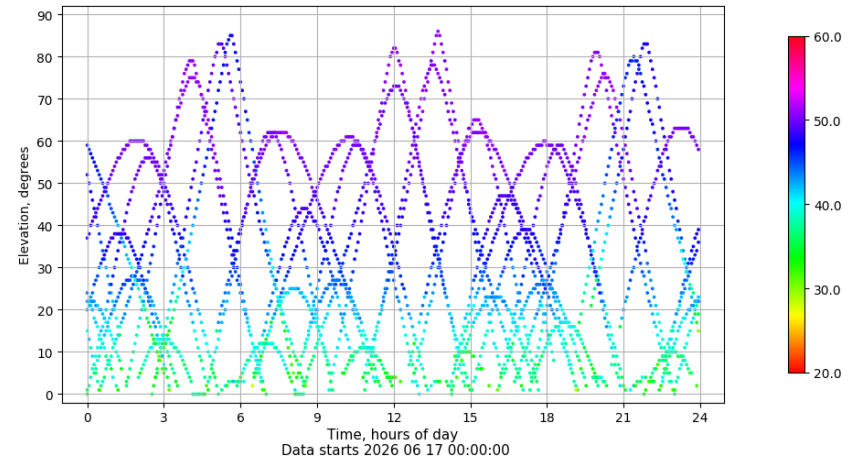
Time-elevation plot for station BCL1. Signal to Noise S1C Data file BCL100ESP_R_2026168.xtr
