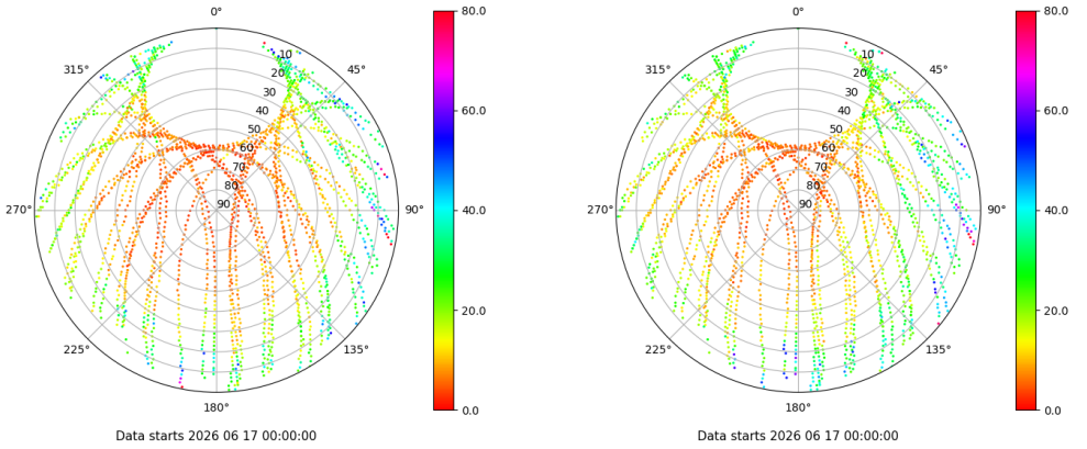
Skyplot for station BCL1. Parameter M1C Data file BCL100ESP_R_2026168.xtr Skyplot for station BCL1. Parameter M2P Data file BCL100ESP_R_2026168.xtr
