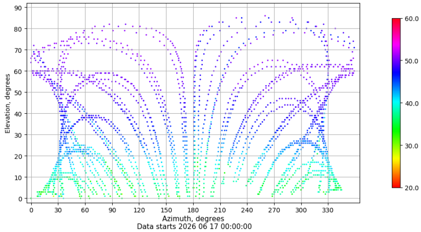
Azimuth-elevation plot for station BCL1. Signal to Noise S1C Data file BCL100ESP_R_2026168.xtr
