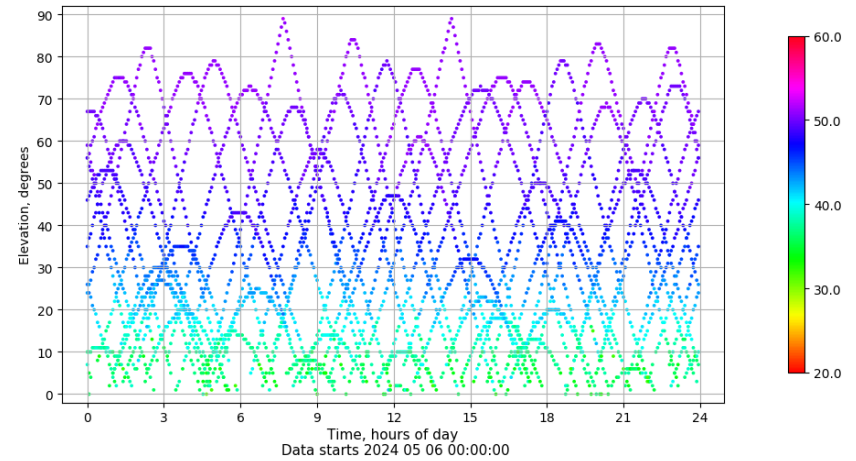
Time-elevation plot for station BCL1. Signal to Noise S1C Data file BCL100ESP_R_2024127.xtr
