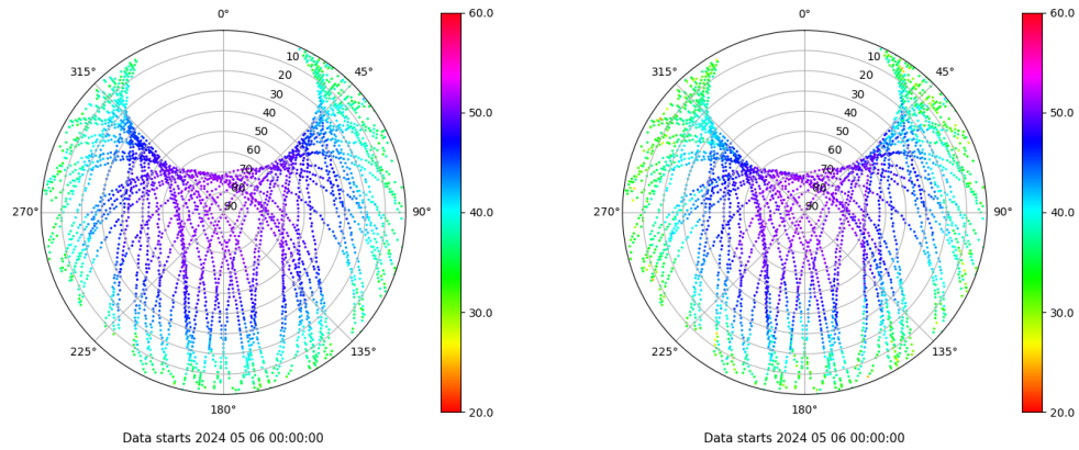
Skyplot for station BCL1. Signal to Noise S1C Data file BCL100ESP_R_2024127.xtr Skyplot for station BCL1. Signal to Noise S2W Data file BCL100ESP_R_2024127.xtr
