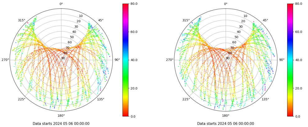
Skyplot for station BCL1. Parameter M1C Data file BCL100ESP_R_2024127.xtr Skyplot for station BCL1. Parameter M2W Data file BCL100ESP_R_2024127.xtr
