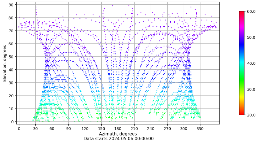
Azimuth-elevation plot for station BCL1. Signal to Noise S1C Data file BCL100ESP_R_2024127.xtr
