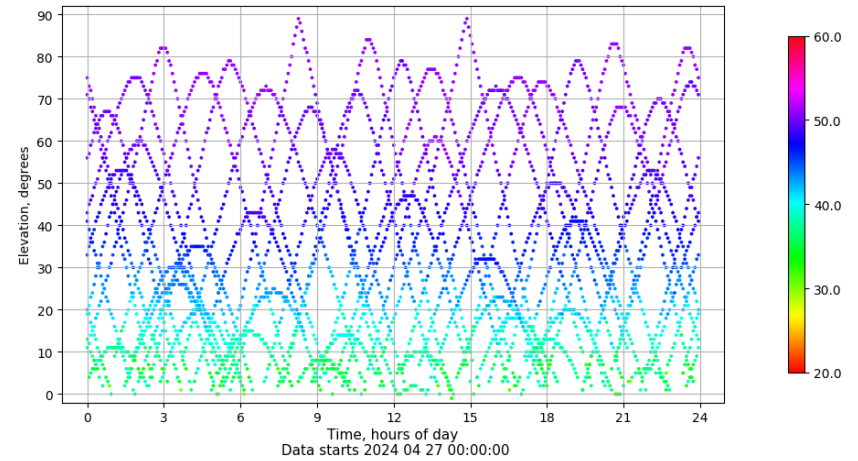
Time-elevation plot for station BCL1. Signal to Noise S1C Data file BCL100ESP_R_2024118.xtr
