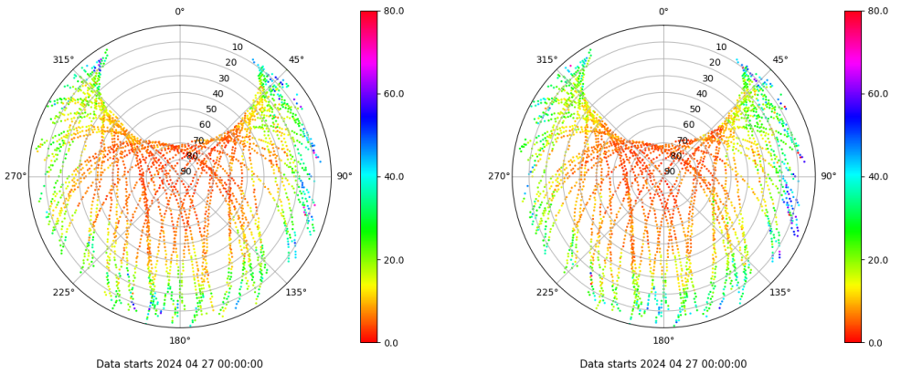
Skyplot for station BCL1. Parameter M1C Data file BCL100ESP_R_2024118.xtr Skyplot for station BCL1. Parameter M2W Data file BCL100ESP_R_2024118.xtr
