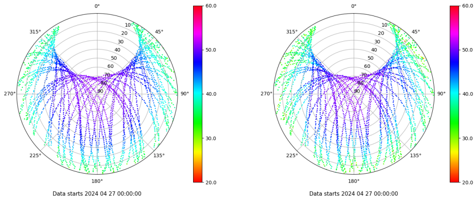
Skyplot for station BCL1. Signal to Noise S1C Data file BCL100ESP_R_2024118.xtr Skyplot for station BCL1. Signal to Noise S2W Data file BCL100ESP_R_2024118.xtr
