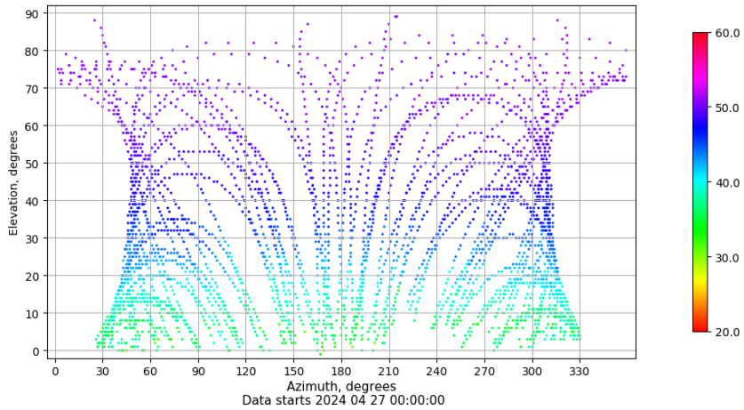
Azimuth-elevation plot for station BCL1. Signal to Noise S1C Data file BCL100ESP_R_2024118.xtr
