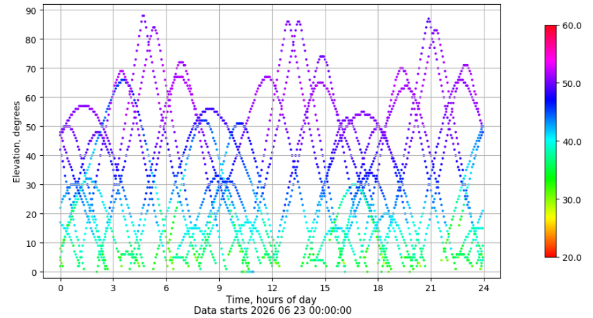
Time-elevation plot for station BADI. Signal to Noise S1C Data file BADI00ESP_R_2026174.xtr
