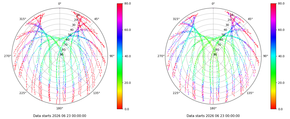
Skyplot for station BADI. Parameter M1C Data file BADI00ESP_R_2026174.xtr Skyplot for station BADI. Parameter M2C Data file BADI00ESP_R_2026174.xtr
