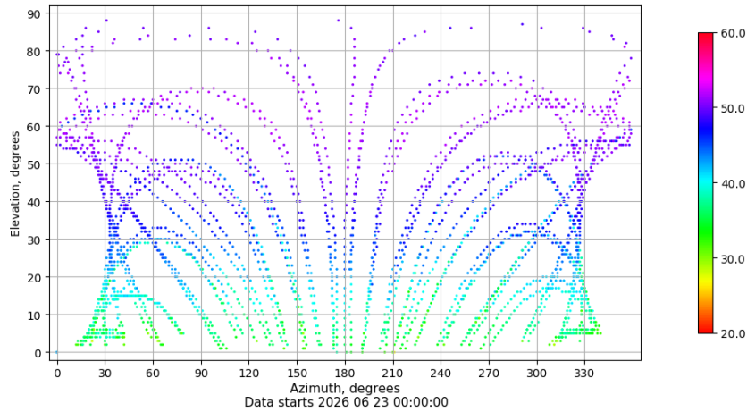
Azimuth-elevation plot for station BADI. Signal to Noise S1C Data file BADI00ESP_R_2026174.xtr
