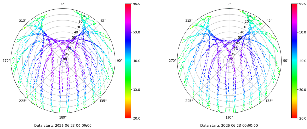
Skyplot for station BADI. Signal to Noise S1C Data file BADI00ESP_R_2026174.xtr Skyplot for station BADI. Signal to Noise S2C Data file BADI00ESP_R_2026174.xtr
