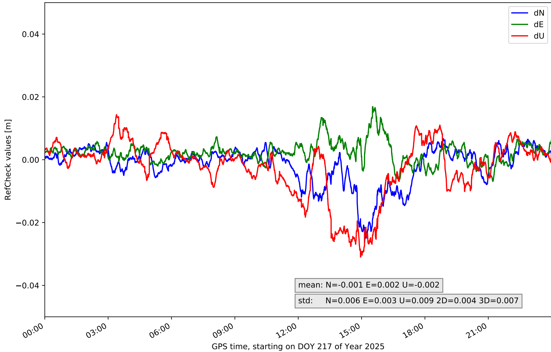
RefCheck for station BADI in network NET2
