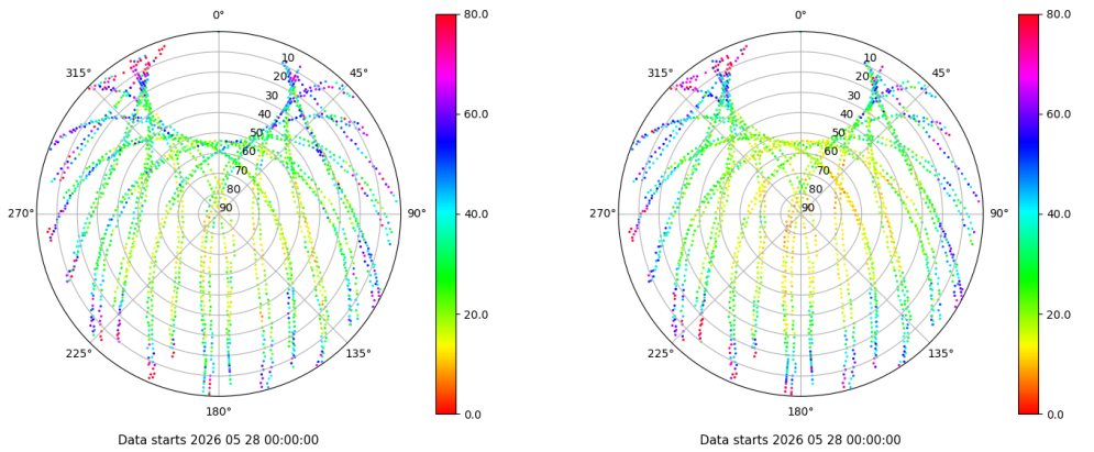
Skyplot for station ZFRA. Parameter M1C Data file ZFRA00ESP_R_2026148.xtr Skyplot for station ZFRA. Parameter M2P Data file ZFRA00ESP_R_2026148.xtr
