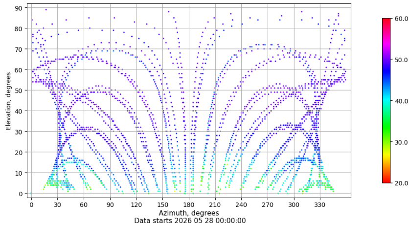
Azimuth-elevation plot for station ZFRA. Signal to Noise S1C Data file ZFRA00ESP_R_2026148.xtr
