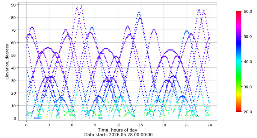
Time-elevation plot for station ZFRA. Signal to Noise S1C Data file ZFRA00ESP_R_2026148.xtr
