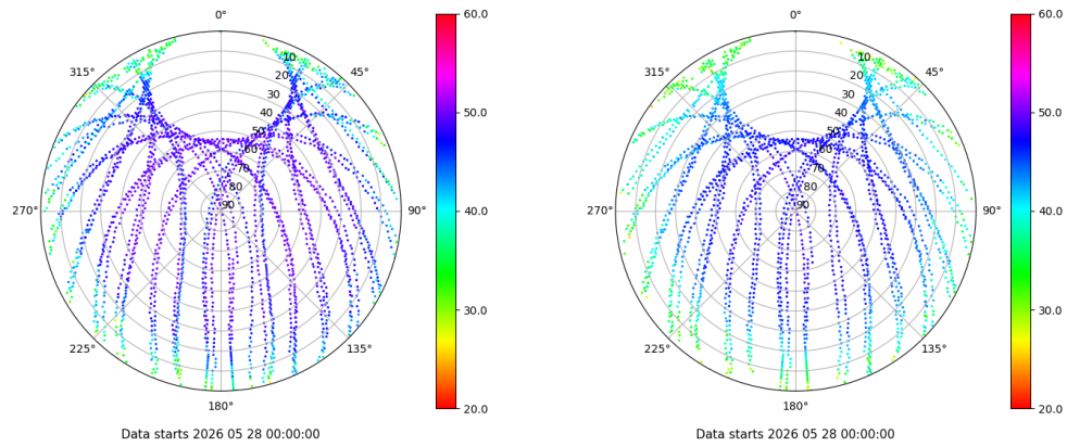
Skyplot for station ZFRA. Signal to Noise S1C Data file ZFRA00ESP_R_2026148.xtr Skyplot for station ZFRA. Signal to Noise S2P Data file ZFRA00ESP_R_2026148.xtr
