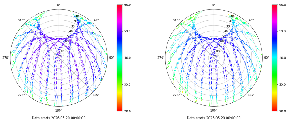
Skyplot for station ZFRA. Signal to Noise S1C Data file ZFRA00ESP_R_2026140.xtr Skyplot for station ZFRA. Signal to Noise S2P Data file ZFRA00ESP_R_2026140.xtr
