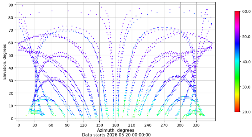
Azimuth-elevation plot for station ZFRA. Signal to Noise S1C Data file ZFRA00ESP_R_2026140.xtr
