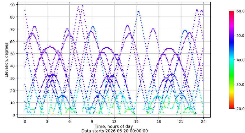
Time-elevation plot for station ZFRA. Signal to Noise S1C Data file ZFRA00ESP_R_2026140.xtr
