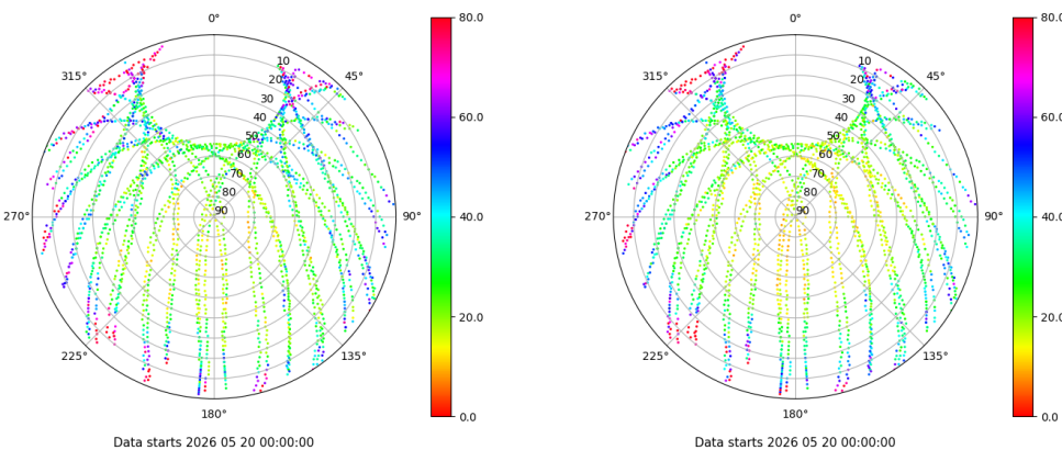
Skyplot for station ZFRA. Parameter M1C Data file ZFRA00ESP_R_2026140.xtr Skyplot for station ZFRA. Parameter M2P Data file ZFRA00ESP_R_2026140.xtr
