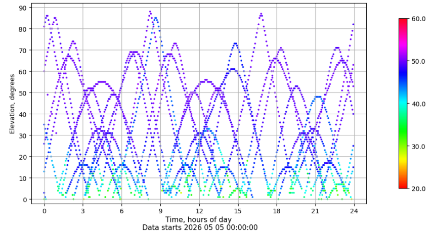
Time-elevation plot for station ZFRA. Signal to Noise S1C Data file ZFRA00ESP_R_2026125.xtr
