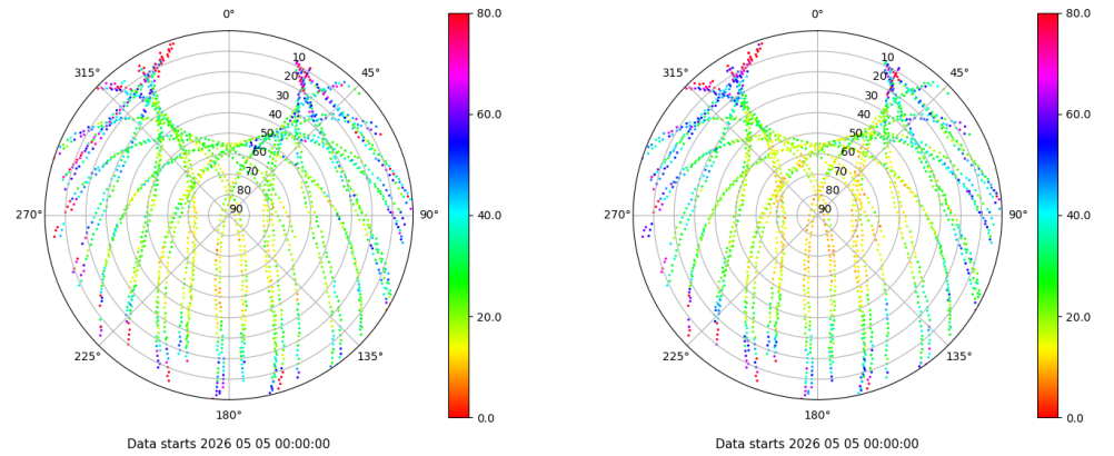
Skyplot for station ZFRA. Parameter M1C Data file ZFRA00ESP_R_2026125.xtr Skyplot for station ZFRA. Parameter M2P Data file ZFRA00ESP_R_2026125.xtr
