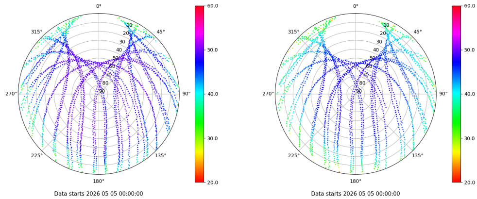
Skyplot for station ZFRA. Signal to Noise S1C Data file ZFRA00ESP_R_2026125.xtr Skyplot for station ZFRA. Signal to Noise S2P Data file ZFRA00ESP_R_2026125.xtr
