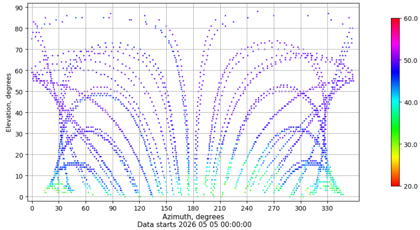
Azimuth-elevation plot for station ZFRA. Signal to Noise S1C Data file ZFRA00ESP_R_2026125.xtr
