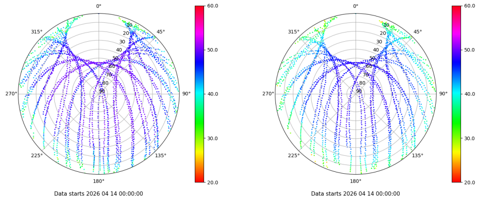
Skyplot for station ZFRA. Signal to Noise S1C Data file ZFRA00ESP_R_2026104.xtr Skyplot for station ZFRA. Signal to Noise S2P Data file ZFRA00ESP_R_2026104.xtr
