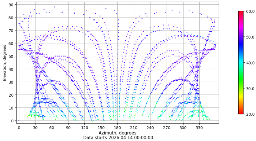
Azimuth-elevation plot for station ZFRA. Signal to Noise S1C Data file ZFRA00ESP_R_2026104.xtr
