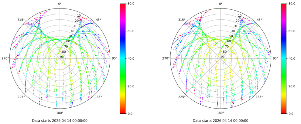
Skyplot for station ZFRA. Parameter M1C Data file ZFRA00ESP_R_2026104.xtr Skyplot for station ZFRA. Parameter M2P Data file ZFRA00ESP_R_2026104.xtr
