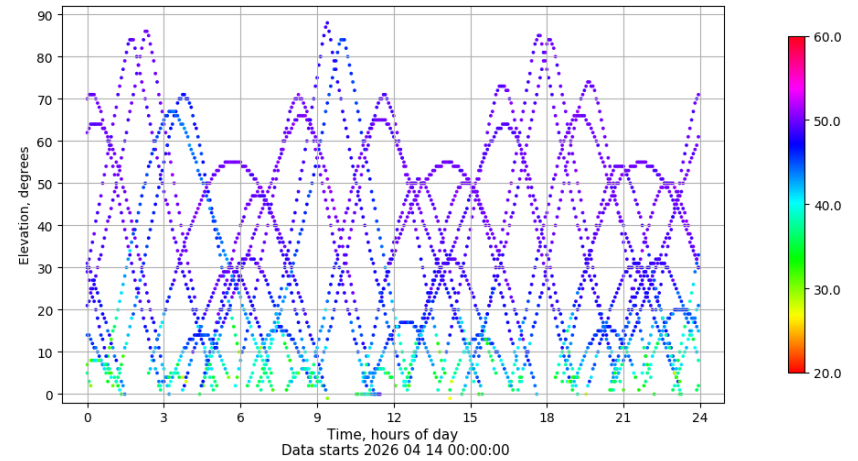
Time-elevation plot for station ZFRA. Signal to Noise S1C Data file ZFRA00ESP_R_2026104.xtr
