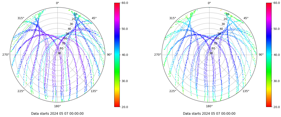
Skyplot for station ZFRA. Signal to Noise S1C Data file ZFRA00ESP_R_2024128.xtr Skyplot for station ZFRA. Signal to Noise S2P Data file ZFRA00ESP_R_2024128.xtr
