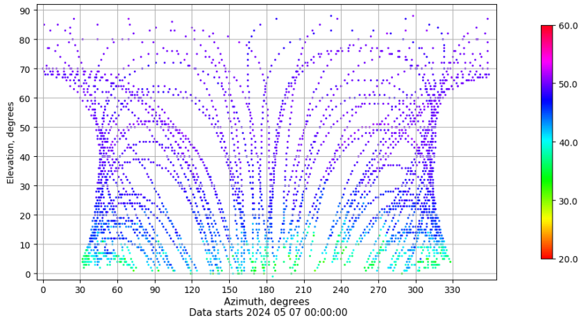
Azimuth-elevation plot for station ZFRA. Signal to Noise S1C Data file ZFRA00ESP_R_2024128.xtr
