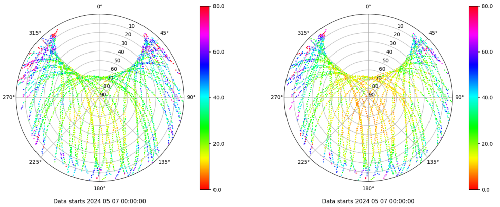
Skyplot for station ZFRA. Parameter M1C Data file ZFRA00ESP_R_2024128.xtr Skyplot for station ZFRA. Parameter M2W Data file ZFRA00ESP_R_2024128.xtr
