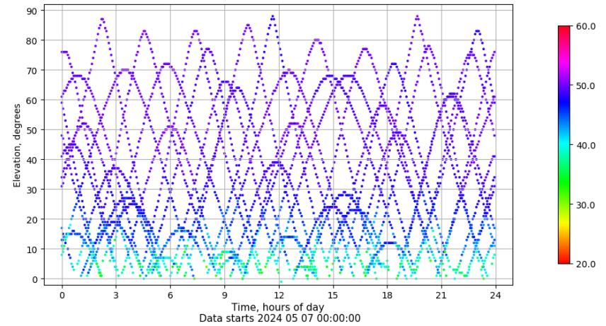
Time-elevation plot for station ZFRA. Signal to Noise S1C Data file ZFRA00ESP_R_2024128.xtr
