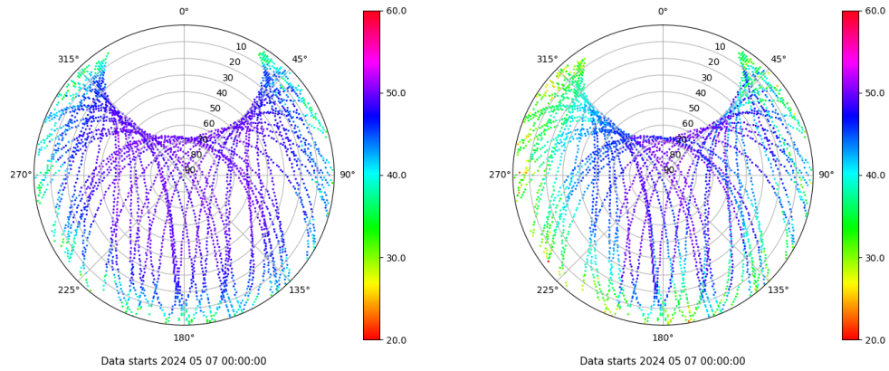
Skyplot for station ZFRA. Signal to Noise S1C Data file ZFRA00ESP_R_2024128.xtr Skyplot for station ZFRA. Signal to Noise S2W Data file ZFRA00ESP_R_2024128.xtr
