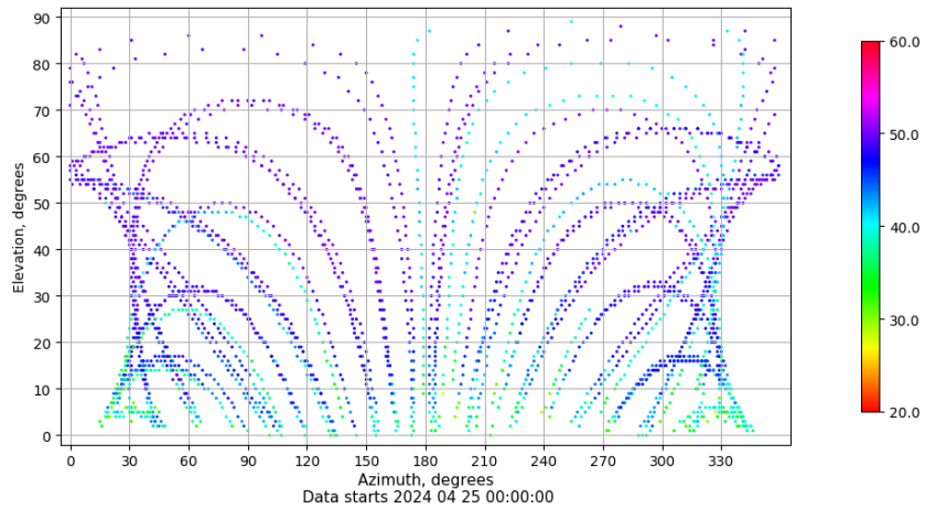
Azimuth-elevation plot for station ZFRA. Signal to Noise S1C Data file ZFRA00ESP_R_2024116.xtr
