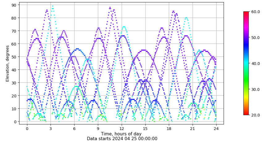
Time-elevation plot for station ZFRA. Signal to Noise S1C Data file ZFRA00ESP_R_2024116.xtr
