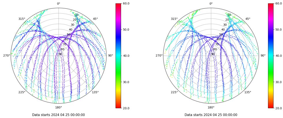
Skyplot for station ZFRA. Signal to Noise S1C Data file ZFRA00ESP_R_2024116.xtr Skyplot for station ZFRA. Signal to Noise S2P Data file ZFRA00ESP_R_2024116.xtr
