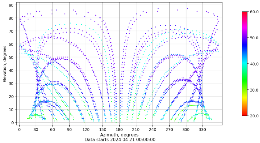
Azimuth-elevation plot for station ZFRA. Signal to Noise S1C Data file ZFRA00ESP_R_2024112.xtr
