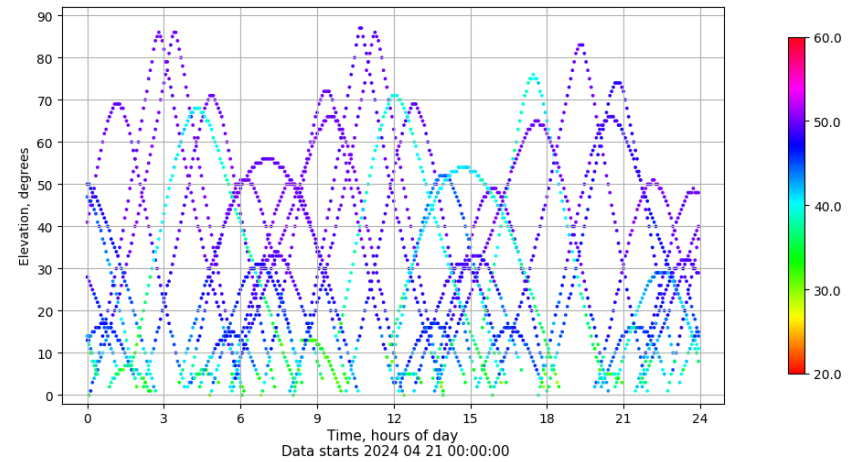
Time-elevation plot for station ZFRA. Signal to Noise S1C Data file ZFRA00ESP_R_2024112.xtr
