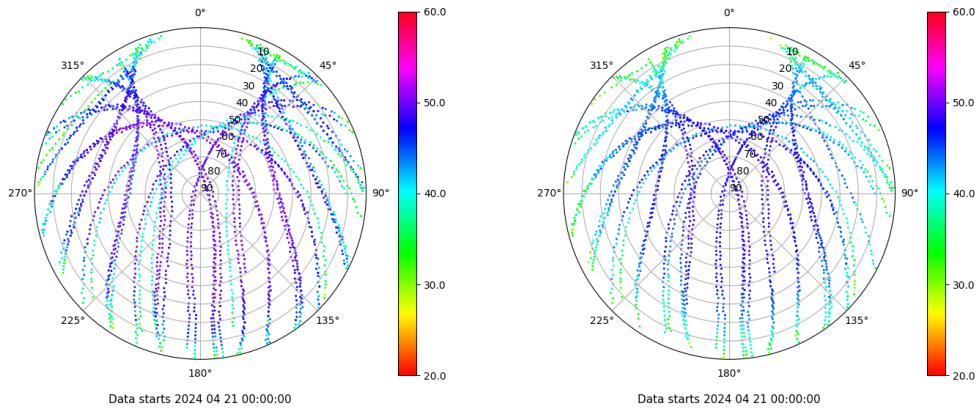
Skyplot for station ZFRA. Signal to Noise S1C Data file ZFRA00ESP_R_2024112.xtr Skyplot for station ZFRA. Signal to Noise S2P Data file ZFRA00ESP_R_2024112.xtr
