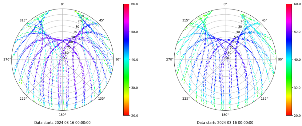
Skyplot for station ZFRA. Signal to Noise S1C Data file ZFRA00ESP_R_2024076.xtr Skyplot for station ZFRA. Signal to Noise S2P Data file ZFRA00ESP_R_2024076.xtr
