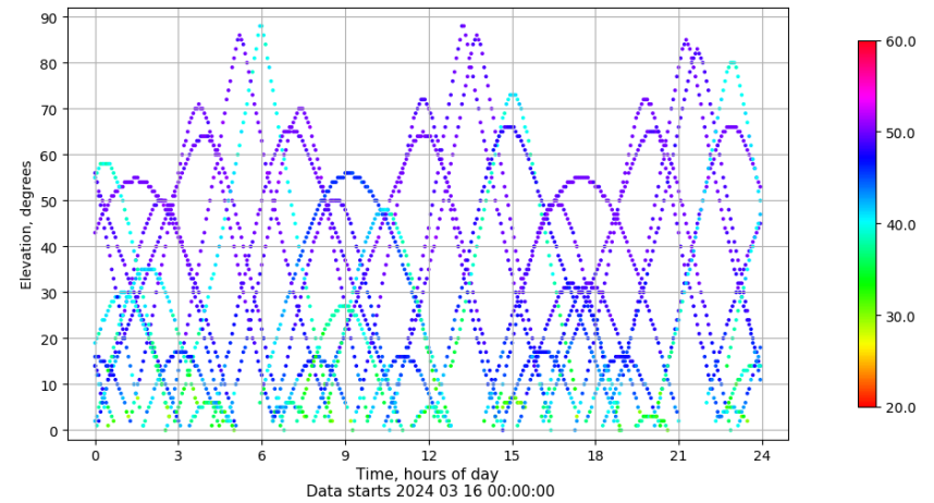
Time-elevation plot for station ZFRA. Signal to Noise S1C Data file ZFRA00ESP_R_2024076.xtr
