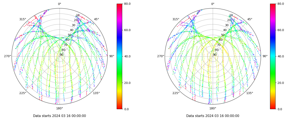
Skyplot for station ZFRA. Parameter M1C Data file ZFRA00ESP_R_2024076.xtr Skyplot for station ZFRA. Parameter M2P Data file ZFRA00ESP_R_2024076.xtr
