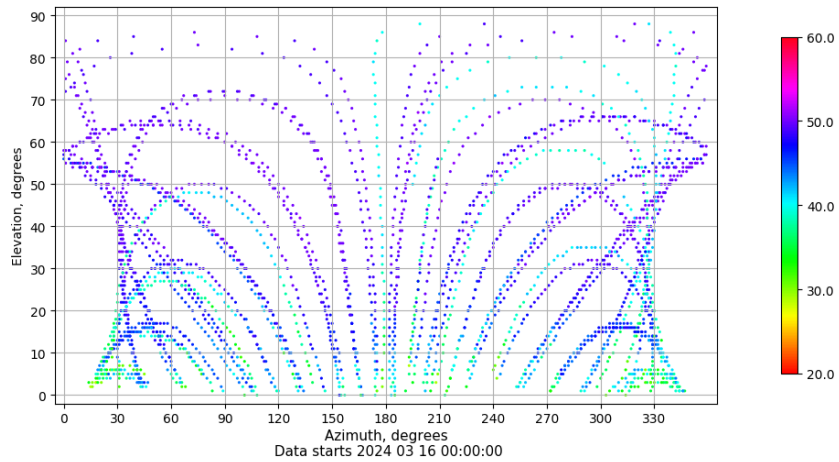
Azimuth-elevation plot for station ZFRA. Signal to Noise S1C Data file ZFRA00ESP_R_2024076.xtr
