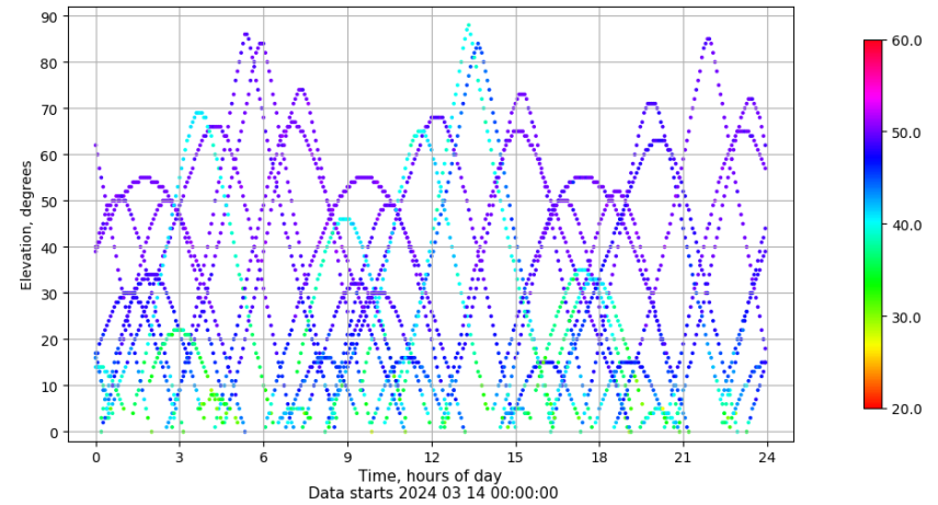
Time-elevation plot for station ZFRA. Signal to Noise S1C Data file ZFRA00ESP_R_2024074.xtr
