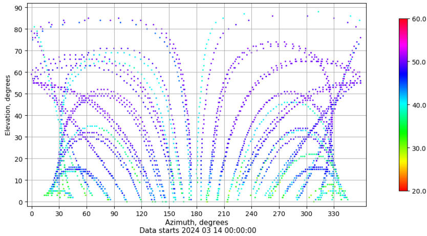
Azimuth-elevation plot for station ZFRA. Signal to Noise S1C Data file ZFRA00ESP_R_2024074.xtr
