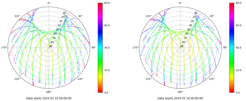
Skyplot for station ZFRA. Parameter M1C Data file ZFRA00ESP_R_2024074.xtr Skyplot for station ZFRA. Parameter M2P Data file ZFRA00ESP_R_2024074.xtr
