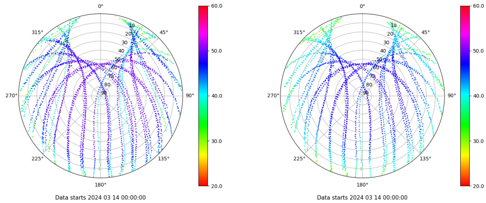
Skyplot for station ZFRA. Signal to Noise S1C Data file ZFRA00ESP_R_2024074.xtr Skyplot for station ZFRA. Signal to Noise S2P Data file ZFRA00ESP_R_2024074.xtr
