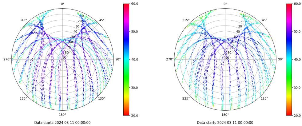
Skyplot for station ZFRA. Signal to Noise S1C Data file ZFRA00ESP_R_2024071.xtr Skyplot for station ZFRA. Signal to Noise S2P Data file ZFRA00ESP_R_2024071.xtr
