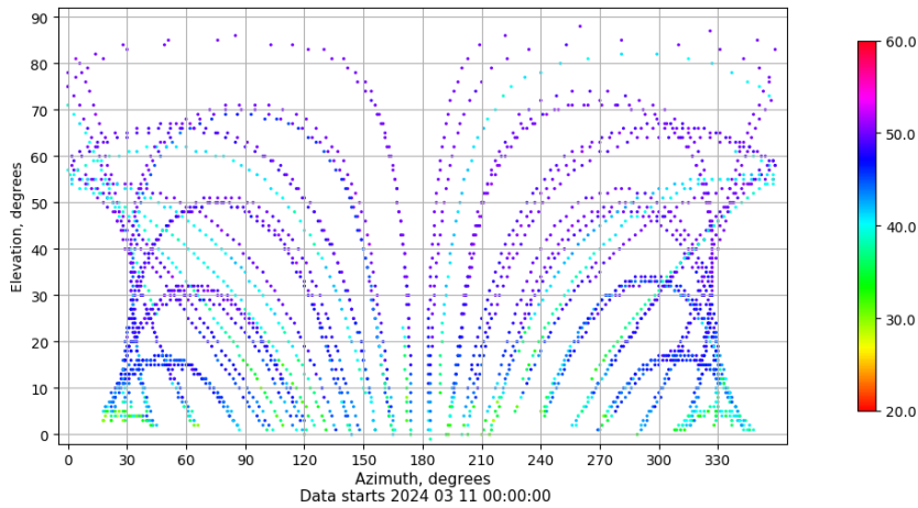
Azimuth-elevation plot for station ZFRA. Signal to Noise S1C Data file ZFRA00ESP_R_2024071.xtr
