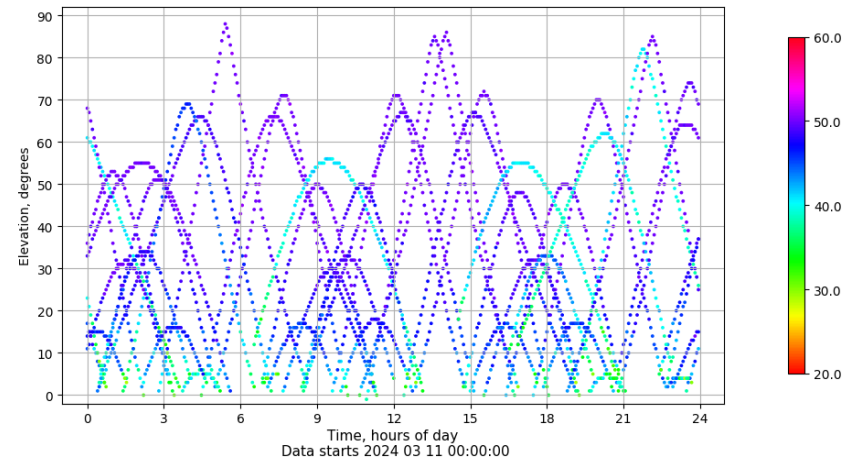
Time-elevation plot for station ZFRA. Signal to Noise S1C Data file ZFRA00ESP_R_2024071.xtr
