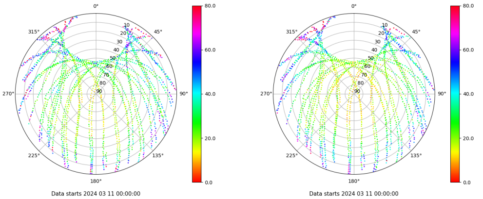
Skyplot for station ZFRA. Parameter M1C Data file ZFRA00ESP_R_2024071.xtr Skyplot for station ZFRA. Parameter M2P Data file ZFRA00ESP_R_2024071.xtr
