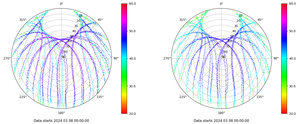
Skyplot for station ZFRA. Signal to Noise S1C Data file ZFRA00ESP_R_2024068.xtr Skyplot for station ZFRA. Signal to Noise S2P Data file ZFRA00ESP_R_2024068.xtr
