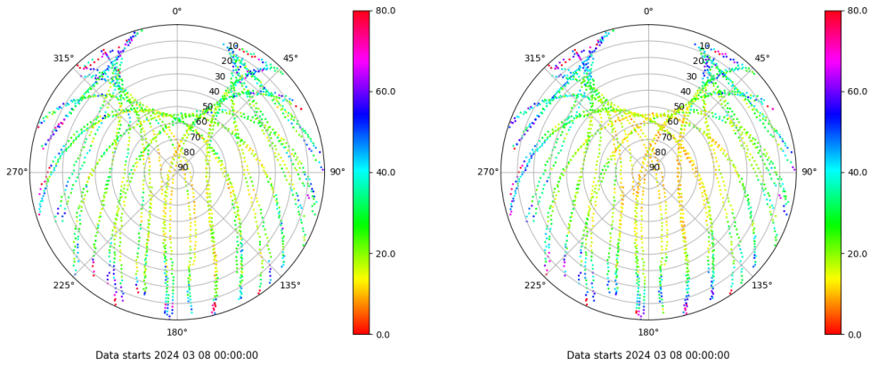
Skyplot for station ZFRA. Parameter M1C Data file ZFRA00ESP_R_2024068.xtr Skyplot for station ZFRA. Parameter M2P Data file ZFRA00ESP_R_2024068.xtr
