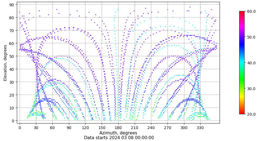
Azimuth-elevation plot for station ZFRA. Signal to Noise S1C Data file ZFRA00ESP_R_2024068.xtr
