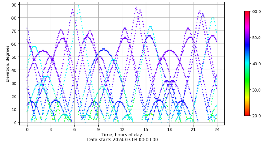
Time-elevation plot for station ZFRA. Signal to Noise S1C Data file ZFRA00ESP_R_2024068.xtr
