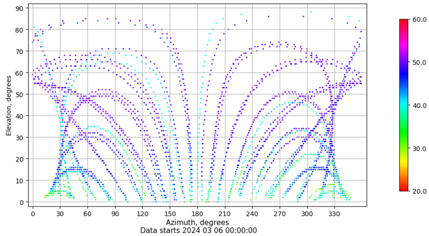
Azimuth-elevation plot for station ZFRA. Signal to Noise S1C Data file ZFRA00ESP_R_2024066.xtr
