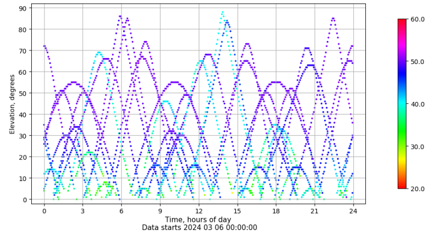
Time-elevation plot for station ZFRA. Signal to Noise S1C Data file ZFRA00ESP_R_2024066.xtr
