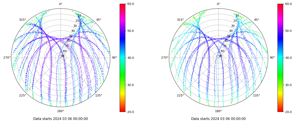
Skyplot for station ZFRA. Signal to Noise S1C Data file ZFRA00ESP_R_2024066.xtr Skyplot for station ZFRA. Signal to Noise S2P Data file ZFRA00ESP_R_2024066.xtr
