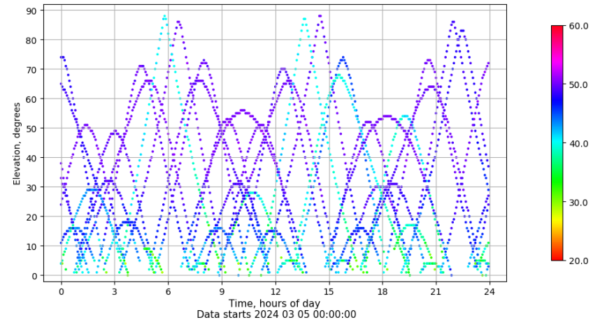
Time-elevation plot for station ZFRA. Signal to Noise S1C Data file ZFRA00ESP_R_2024065.xtr
