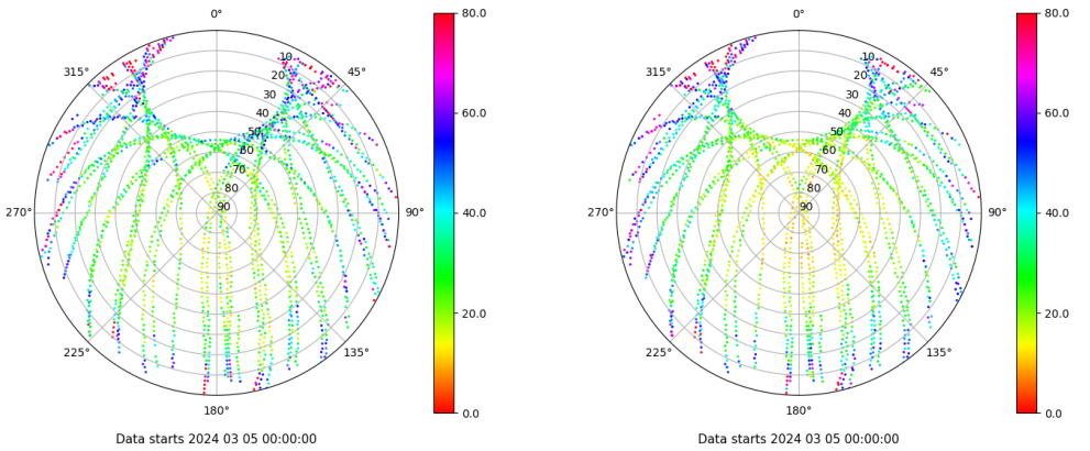
Skyplot for station ZFRA. Parameter M1C Data file ZFRA00ESP_R_2024065.xtr Skyplot for station ZFRA. Parameter M2P Data file ZFRA00ESP_R_2024065.xtr
