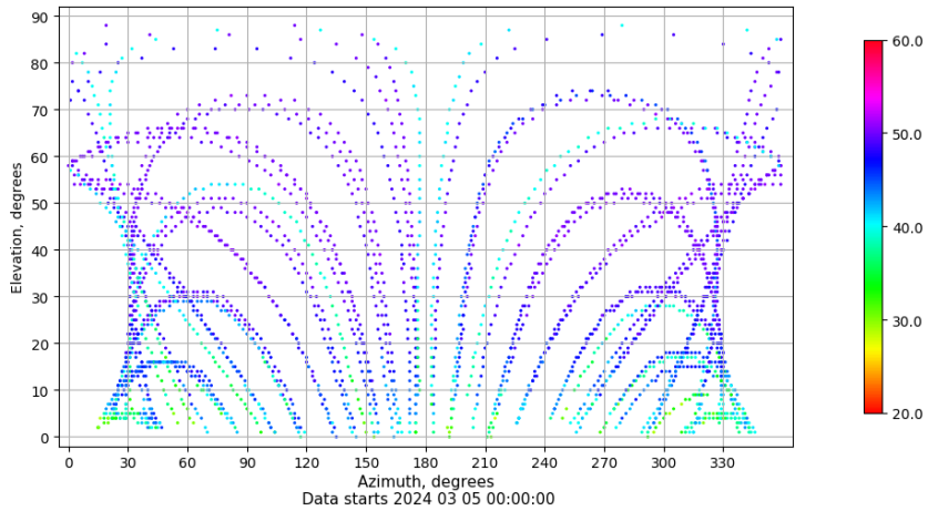
Azimuth-elevation plot for station ZFRA. Signal to Noise S1C Data file ZFRA00ESP_R_2024065.xtr
