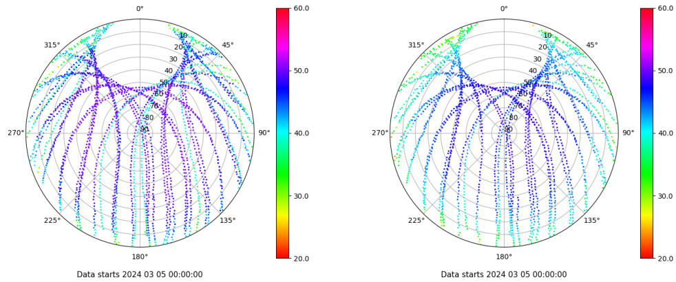
Skyplot for station ZFRA. Signal to Noise S1C Data file ZFRA00ESP_R_2024065.xtr Skyplot for station ZFRA. Signal to Noise S2P Data file ZFRA00ESP_R_2024065.xtr
