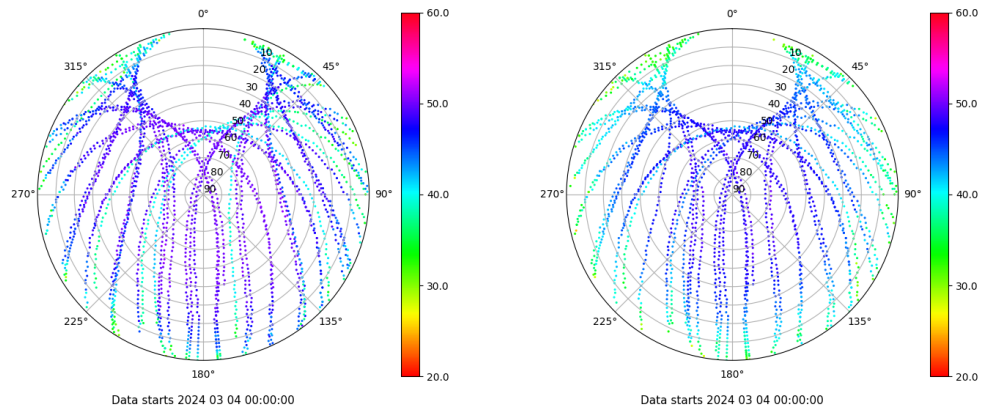
Skyplot for station ZFRA. Signal to Noise S1C Data file ZFRA00ESP_R_2024064.xtr Skyplot for station ZFRA. Signal to Noise S2P Data file ZFRA00ESP_R_2024064.xtr
