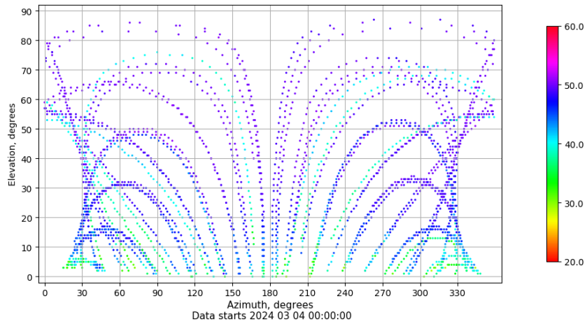
Azimuth-elevation plot for station ZFRA. Signal to Noise S1C Data file ZFRA00ESP_R_2024064.xtr
