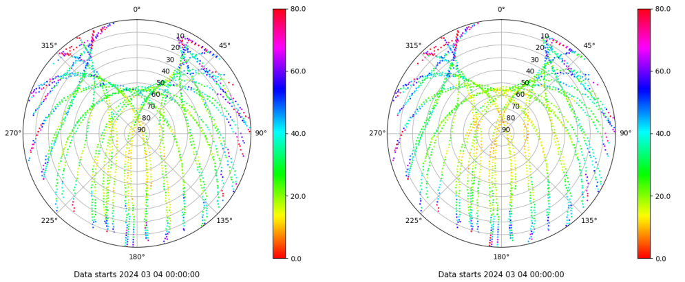
Skyplot for station ZFRA. Parameter M1C Data file ZFRA00ESP_R_2024064.xtr Skyplot for station ZFRA. Parameter M2P Data file ZFRA00ESP_R_2024064.xtr
