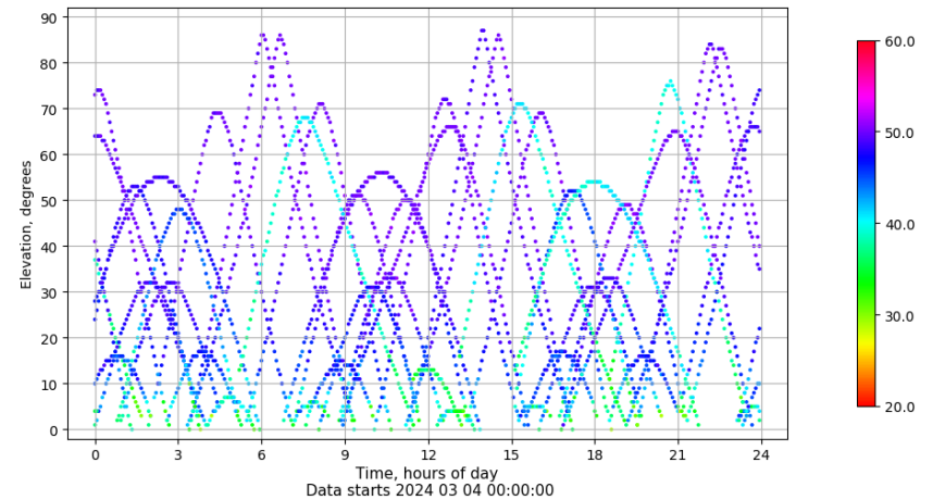
Time-elevation plot for station ZFRA. Signal to Noise S1C Data file ZFRA00ESP_R_2024064.xtr
