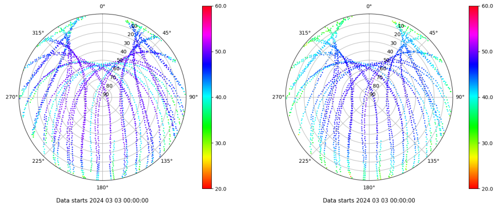
Skyplot for station ZFRA. Signal to Noise S1C Data file ZFRA00ESP_R_2024063.xtr Skyplot for station ZFRA. Signal to Noise S2P Data file ZFRA00ESP_R_2024063.xtr
