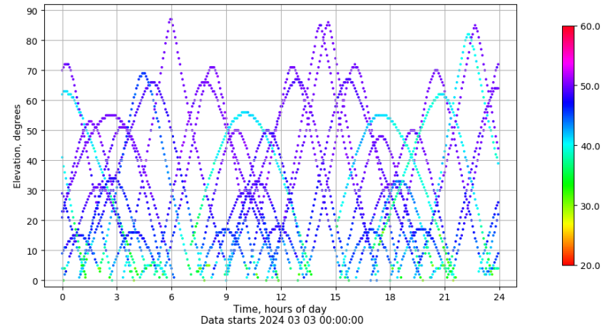
Time-elevation plot for station ZFRA. Signal to Noise S1C Data file ZFRA00ESP_R_2024063.xtr
