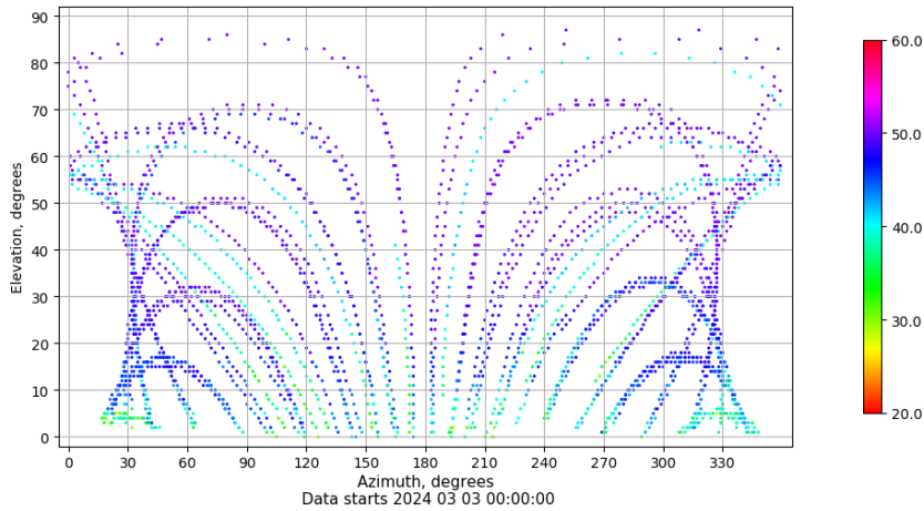
Azimuth-elevation plot for station ZFRA. Signal to Noise S1C Data file ZFRA00ESP_R_2024063.xtr
