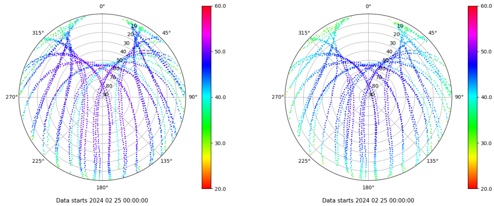
Skyplot for station ZFRA. Signal to Noise S1C Data file ZFRA00ESP_R_2024056.xtr Skyplot for station ZFRA. Signal to Noise S2P Data file ZFRA00ESP_R_2024056.xtr
