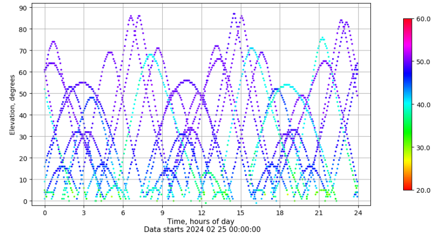
Time-elevation plot for station ZFRA. Signal to Noise S1C Data file ZFRA00ESP_R_2024056.xtr
