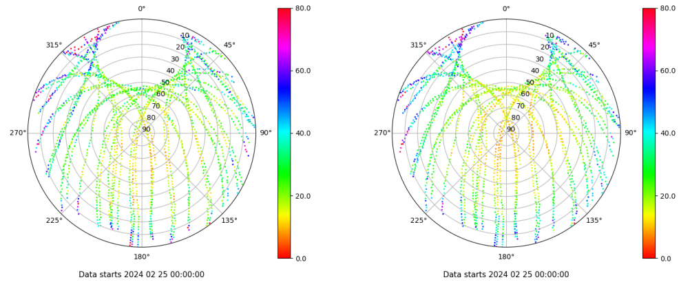
Skyplot for station ZFRA. Parameter M1C Data file ZFRA00ESP_R_2024056.xtr Skyplot for station ZFRA. Parameter M2P Data file ZFRA00ESP_R_2024056.xtr
