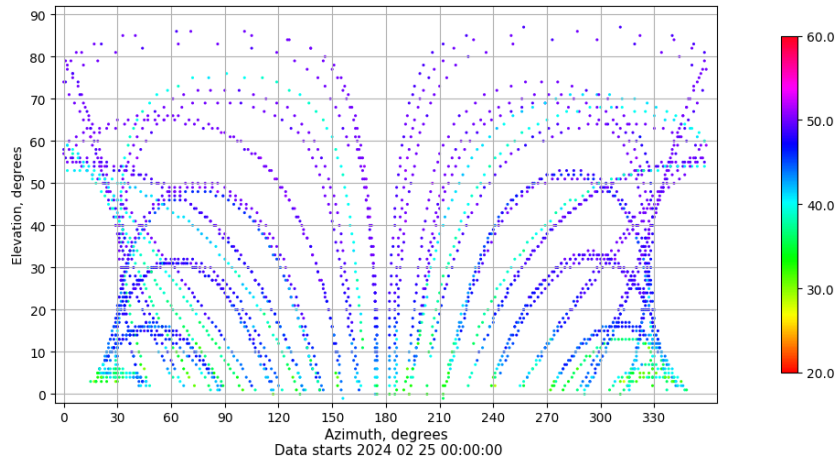
Azimuth-elevation plot for station ZFRA. Signal to Noise S1C Data file ZFRA00ESP_R_2024056.xtr
