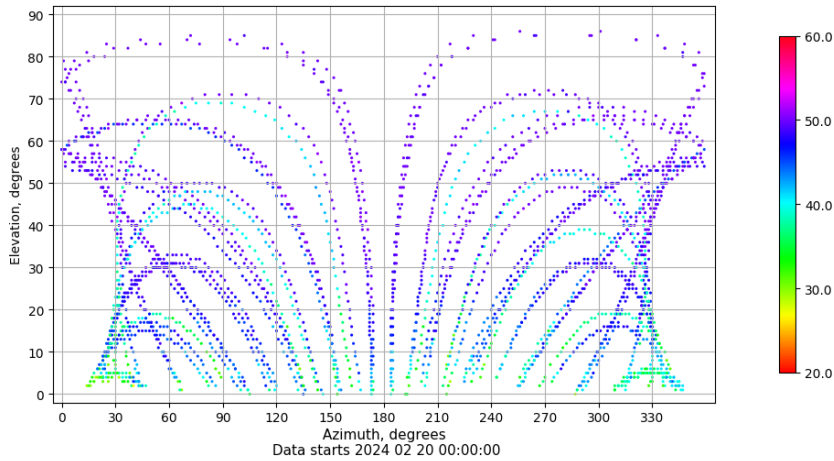
Azimuth-elevation plot for station ZFRA. Signal to Noise S1C Data file ZFRA00ESP_R_2024051.xtr
