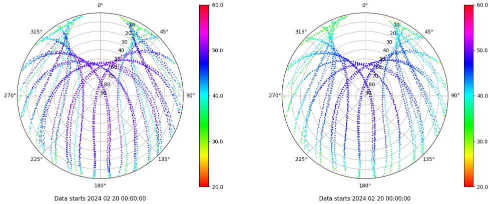
Skyplot for station ZFRA. Signal to Noise S1C Data file ZFRA00ESP_R_2024051.xtr Skyplot for station ZFRA. Signal to Noise S2P Data file ZFRA00ESP_R_2024051.xtr
