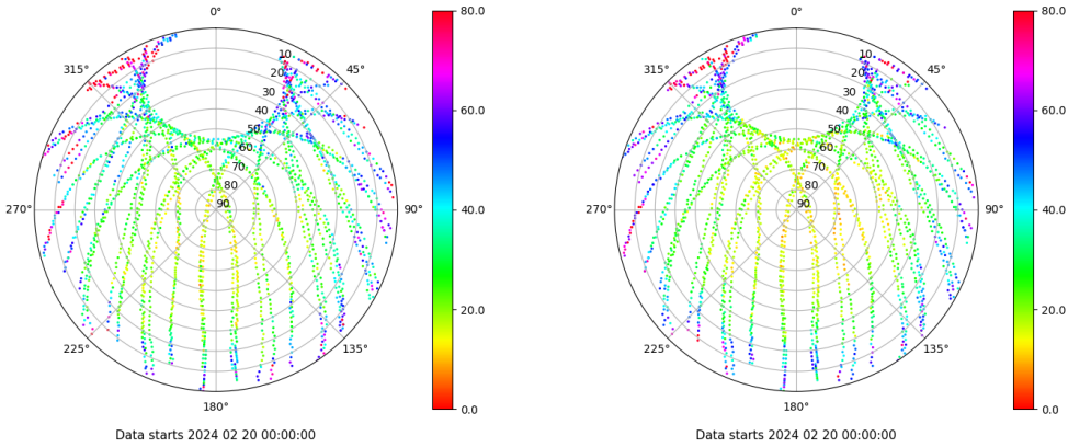
Skyplot for station ZFRA. Parameter M1C Data file ZFRA00ESP_R_2024051.xtr Skyplot for station ZFRA. Parameter M2P Data file ZFRA00ESP_R_2024051.xtr
