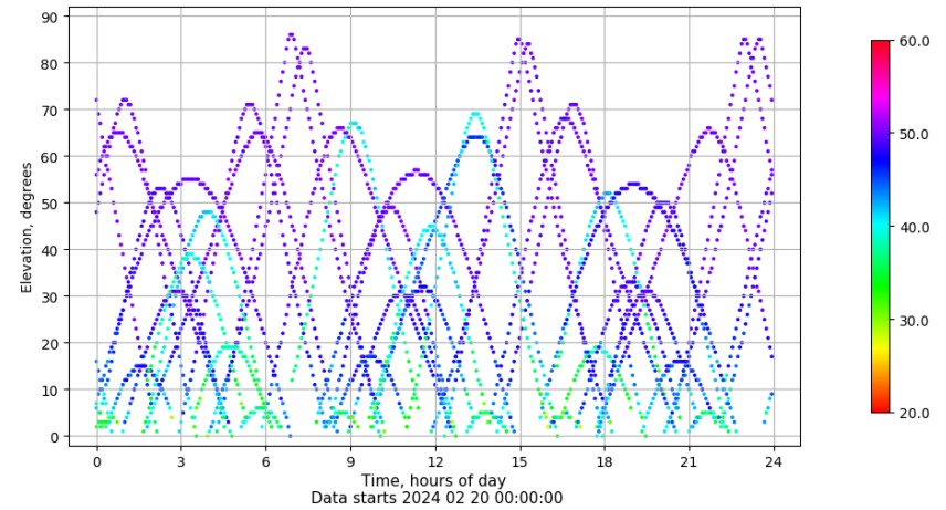
Time-elevation plot for station ZFRA. Signal to Noise S1C Data file ZFRA00ESP_R_2024051.xtr
