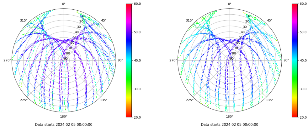
Skyplot for station ZFRA. Signal to Noise S1C Data file ZFRA00ESP_R_2024036.xtr Skyplot for station ZFRA. Signal to Noise S2P Data file ZFRA00ESP_R_2024036.xtr
