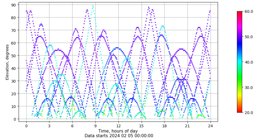
Time-elevation plot for station ZFRA. Signal to Noise S1C Data file ZFRA00ESP_R_2024036.xtr
