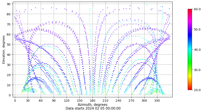
Azimuth-elevation plot for station ZFRA. Signal to Noise S1C Data file ZFRA00ESP_R_2024036.xtr
