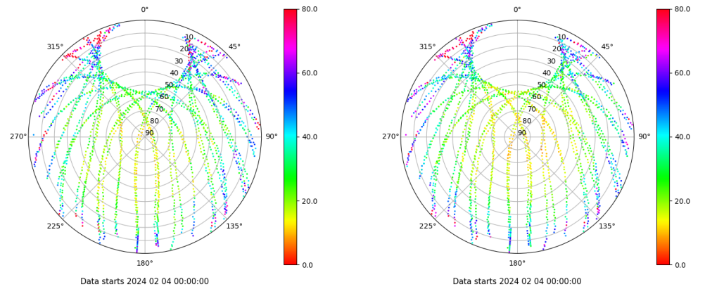
Skyplot for station ZFRA. Parameter M1C Data file ZFRA00ESP_R_2024035.xtr Skyplot for station ZFRA. Parameter M2P Data file ZFRA00ESP_R_2024035.xtr
