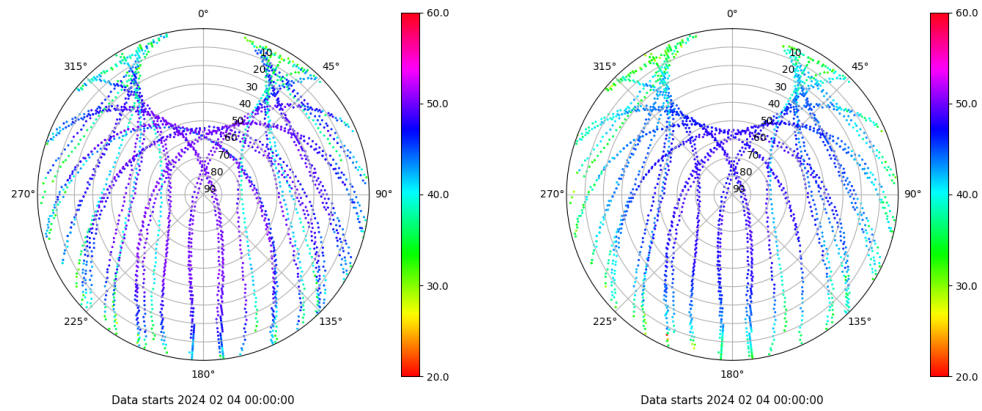
Skyplot for station ZFRA. Signal to Noise S1C Data file ZFRA00ESP_R_2024035.xtr Skyplot for station ZFRA. Signal to Noise S2P Data file ZFRA00ESP_R_2024035.xtr
