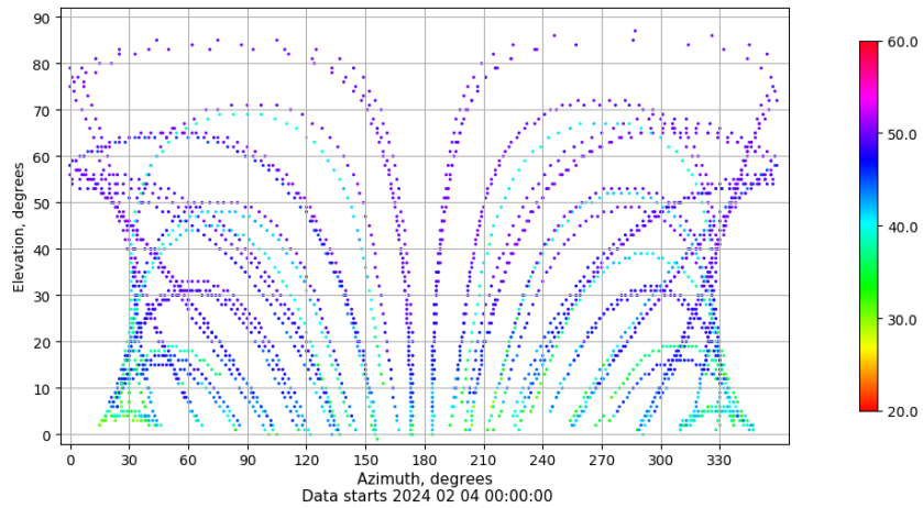
Azimuth-elevation plot for station ZFRA. Signal to Noise S1C Data file ZFRA00ESP_R_2024035.xtr
