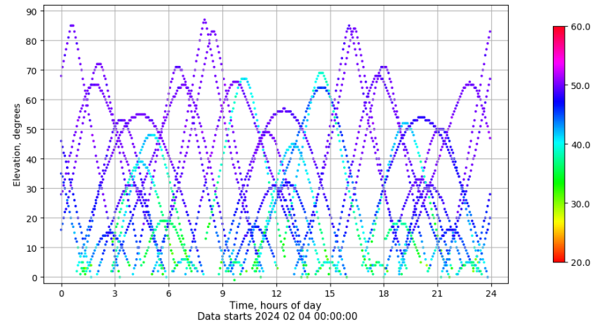
Time-elevation plot for station ZFRA. Signal to Noise S1C Data file ZFRA00ESP_R_2024035.xtr
