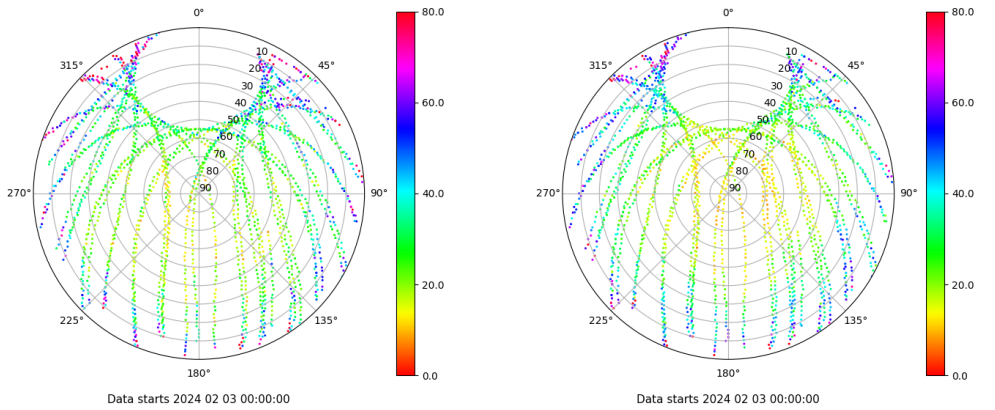
Skyplot for station ZFRA. Parameter M1C Data file ZFRA00ESP_R_2024034.xtr Skyplot for station ZFRA. Parameter M2P Data file ZFRA00ESP_R_2024034.xtr
