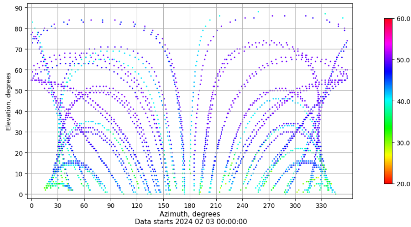
Azimuth-elevation plot for station ZFRA. Signal to Noise S1C Data file ZFRA00ESP_R_2024034.xtr
