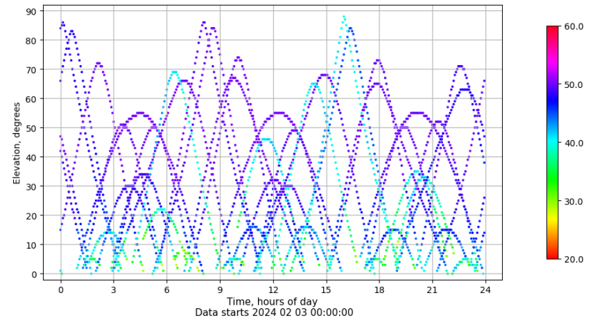
Time-elevation plot for station ZFRA. Signal to Noise S1C Data file ZFRA00ESP_R_2024034.xtr
