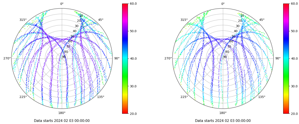
Skyplot for station ZFRA. Signal to Noise S1C Data file ZFRA00ESP_R_2024034.xtr Skyplot for station ZFRA. Signal to Noise S2P Data file ZFRA00ESP_R_2024034.xtr
