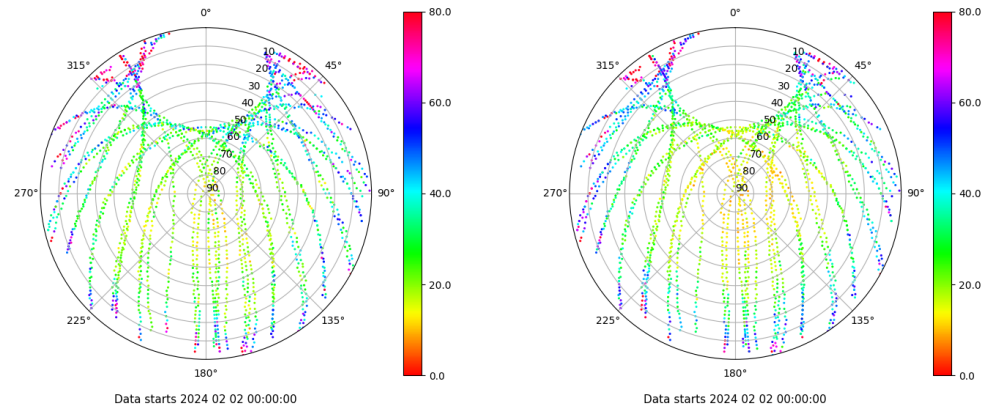
Skyplot for station ZFRA. Parameter M1C Data file ZFRA00ESP_R_2024033.xtr Skyplot for station ZFRA. Parameter M2P Data file ZFRA00ESP_R_2024033.xtr
