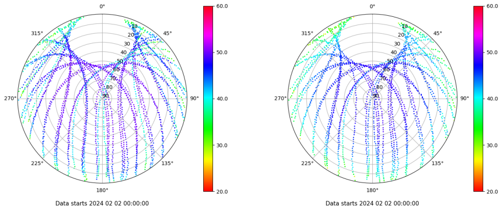
Skyplot for station ZFRA. Signal to Noise S1C Data file ZFRA00ESP_R_2024033.xtr Skyplot for station ZFRA. Signal to Noise S2P Data file ZFRA00ESP_R_2024033.xtr
