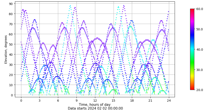
Time-elevation plot for station ZFRA. Signal to Noise S1C Data file ZFRA00ESP_R_2024033.xtr
