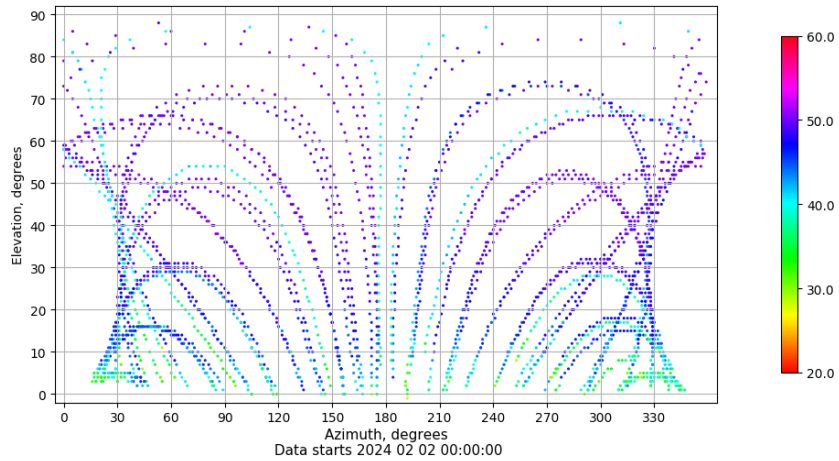
Azimuth-elevation plot for station ZFRA. Signal to Noise S1C Data file ZFRA00ESP_R_2024033.xtr
