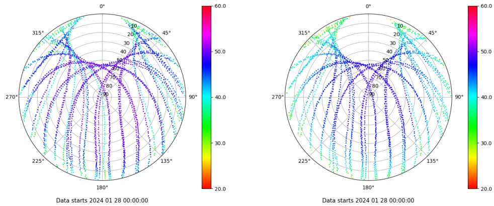
Skyplot for station ZFRA. Signal to Noise S1C Data file ZFRA00ESP_R_2024028.xtr Skyplot for station ZFRA. Signal to Noise S2P Data file ZFRA00ESP_R_2024028.xtr
