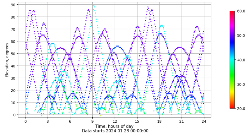
Time-elevation plot for station ZFRA. Signal to Noise S1C Data file ZFRA00ESP_R_2024028.xtr
