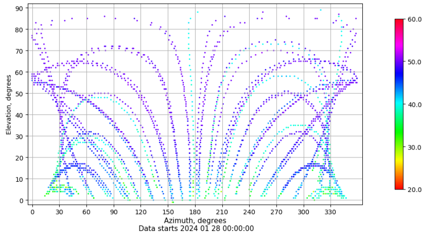
Azimuth-elevation plot for station ZFRA. Signal to Noise S1C Data file ZFRA00ESP_R_2024028.xtr
