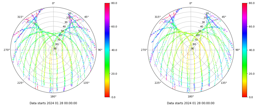
Skyplot for station ZFRA. Parameter M1C Data file ZFRA00ESP_R_2024028.xtr Skyplot for station ZFRA. Parameter M2P Data file ZFRA00ESP_R_2024028.xtr
