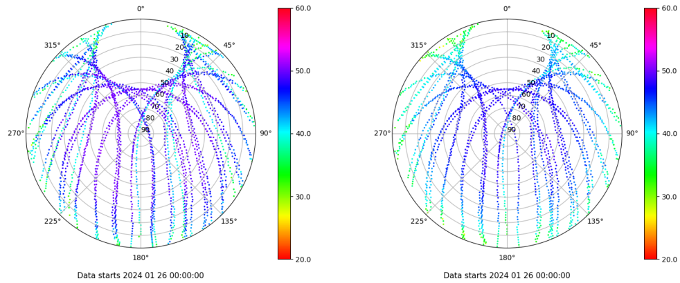
Skyplot for station ZFRA. Signal to Noise S1C Data file ZFRA00ESP_R_2024026.xtr Skyplot for station ZFRA. Signal to Noise S2P Data file ZFRA00ESP_R_2024026.xtr
