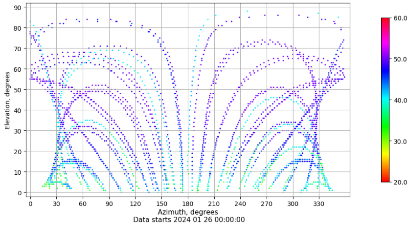
Azimuth-elevation plot for station ZFRA. Signal to Noise S1C Data file ZFRA00ESP_R_2024026.xtr
