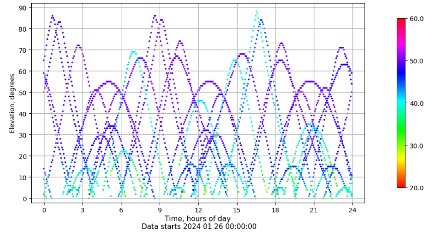
Time-elevation plot for station ZFRA. Signal to Noise S1C Data file ZFRA00ESP_R_2024026.xtr
