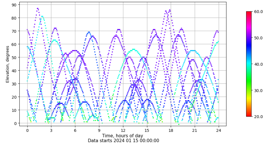
Time-elevation plot for station ZFRA. Signal to Noise S1C Data file ZFRA00ESP_R_2024015.xtr
