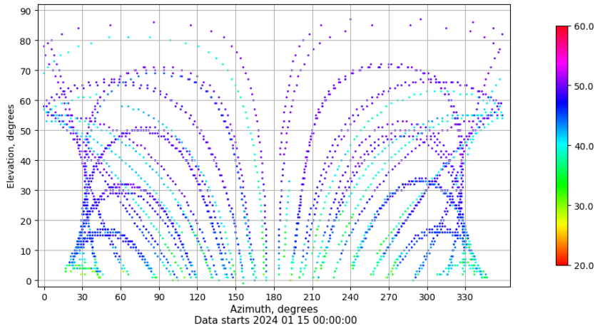
Azimuth-elevation plot for station ZFRA. Signal to Noise S1C Data file ZFRA00ESP_R_2024015.xtr
