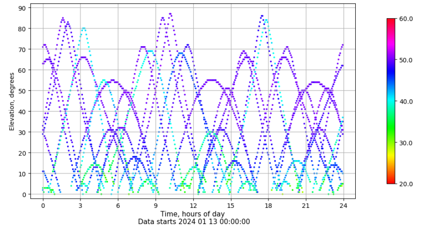
Time-elevation plot for station ZFRA. Signal to Noise S1C Data file ZFRA00ESP_R_2024013.xtr
