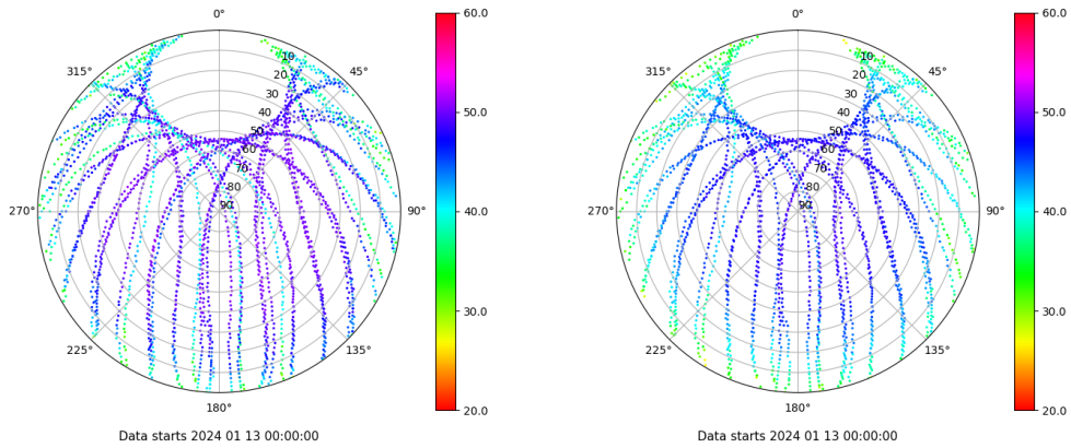
Skyplot for station ZFRA. Signal to Noise S1C Data file ZFRA00ESP_R_2024013.xtr Skyplot for station ZFRA. Signal to Noise S2P Data file ZFRA00ESP_R_2024013.xtr
