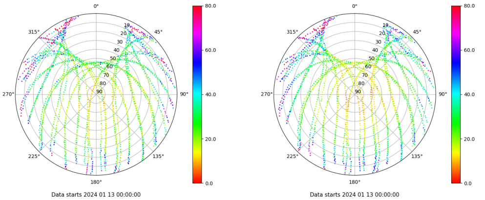
Skyplot for station ZFRA. Parameter M1C Data file ZFRA00ESP_R_2024013.xtr Skyplot for station ZFRA. Parameter M2P Data file ZFRA00ESP_R_2024013.xtr
