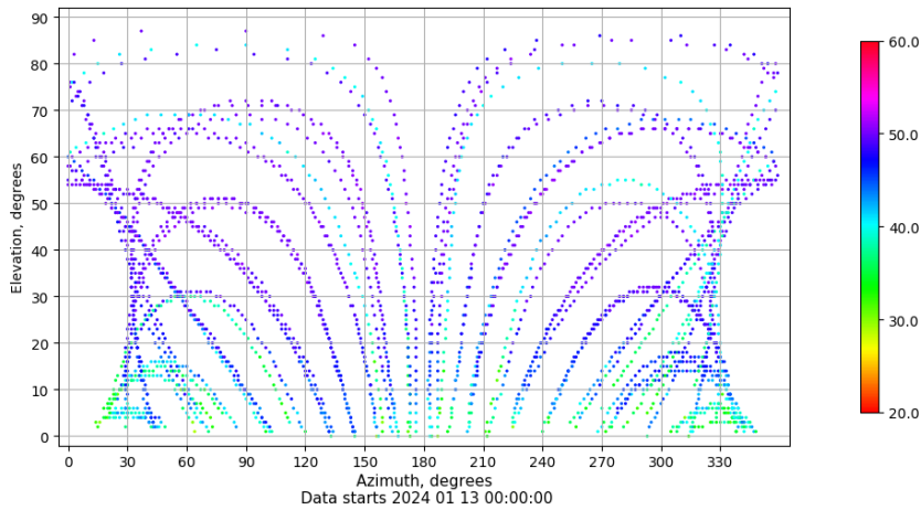
Azimuth-elevation plot for station ZFRA. Signal to Noise S1C Data file ZFRA00ESP_R_2024013.xtr
