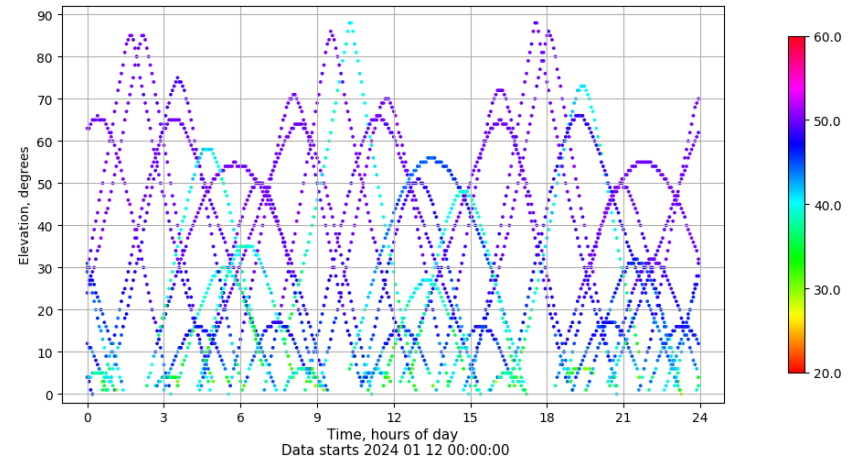
Time-elevation plot for station ZFRA. Signal to Noise S1C Data file ZFRA00ESP_R_2024012.xtr
