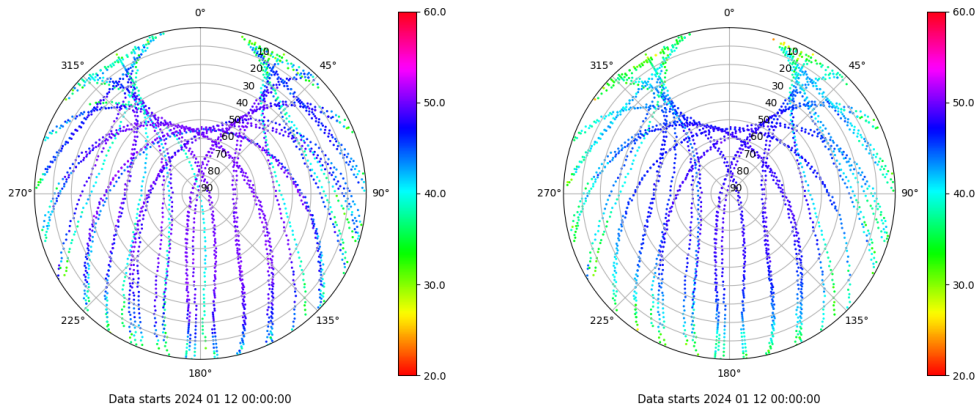
Skyplot for station ZFRA. Signal to Noise S1C Data file ZFRA00ESP_R_2024012.xtr Skyplot for station ZFRA. Signal to Noise S2P Data file ZFRA00ESP_R_2024012.xtr
