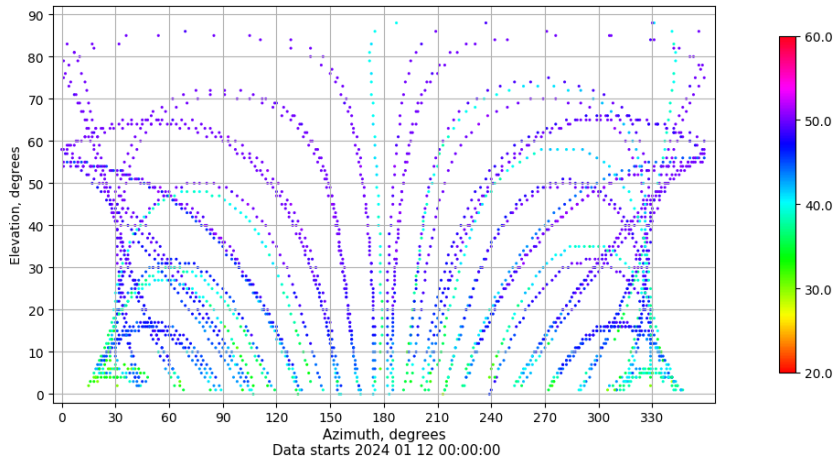
Azimuth-elevation plot for station ZFRA. Signal to Noise S1C Data file ZFRA00ESP_R_2024012.xtr
