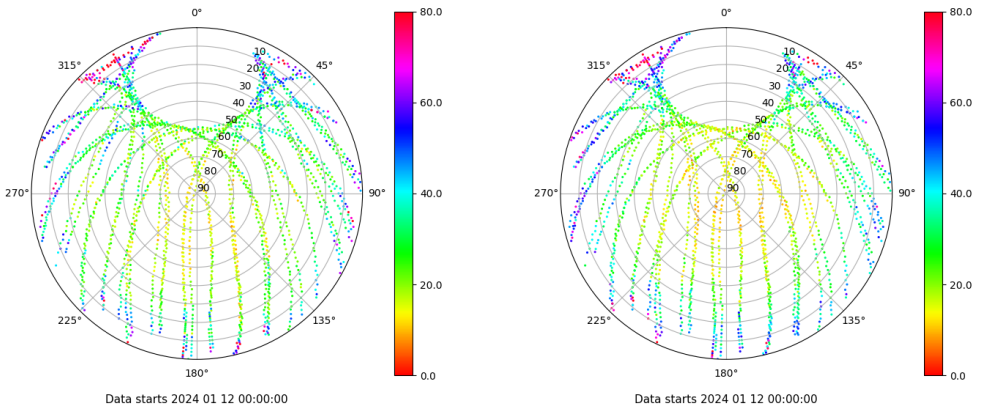
Skyplot for station ZFRA. Parameter M1C Data file ZFRA00ESP_R_2024012.xtr Skyplot for station ZFRA. Parameter M2P Data file ZFRA00ESP_R_2024012.xtr
