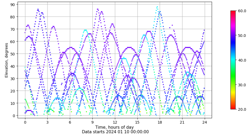
Time-elevation plot for station ZFRA. Signal to Noise S1C Data file ZFRA00ESP_R_2024010.xtr
