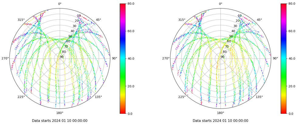
Skyplot for station ZFRA. Parameter M1C Data file ZFRA00ESP_R_2024010.xtr Skyplot for station ZFRA. Parameter M2P Data file ZFRA00ESP_R_2024010.xtr
