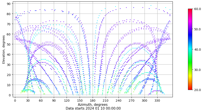
Azimuth-elevation plot for station ZFRA. Signal to Noise S1C Data file ZFRA00ESP_R_2024010.xtr
