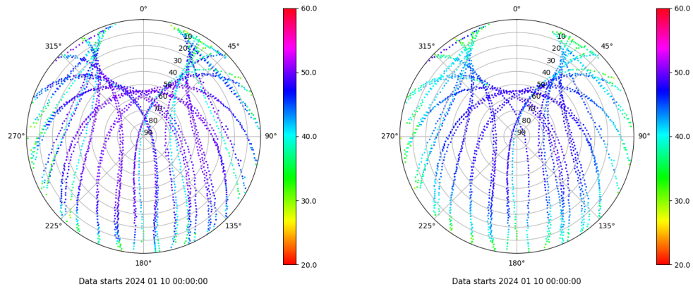
Skyplot for station ZFRA. Signal to Noise S1C Data file ZFRA00ESP_R_2024010.xtr Skyplot for station ZFRA. Signal to Noise S2P Data file ZFRA00ESP_R_2024010.xtr
