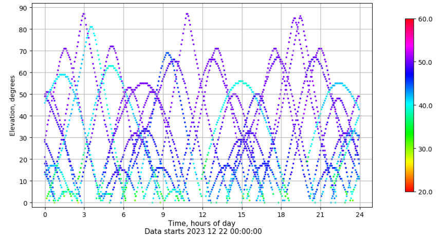
Time-elevation plot for station ZFRA. Signal to Noise S1C Data file ZFRA00ESP_R_2023356.xtr
