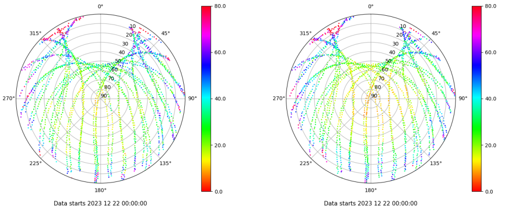
Skyplot for station ZFRA. Parameter M1C Data file ZFRA00ESP_R_2023356.xtr Skyplot for station ZFRA. Parameter M2P Data file ZFRA00ESP_R_2023356.xtr
