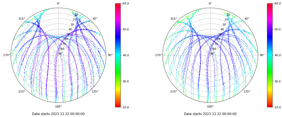
Skyplot for station ZFRA. Signal to Noise S1C Data file ZFRA00ESP_R_2023356.xtr Skyplot for station ZFRA. Signal to Noise S2P Data file ZFRA00ESP_R_2023356.xtr
