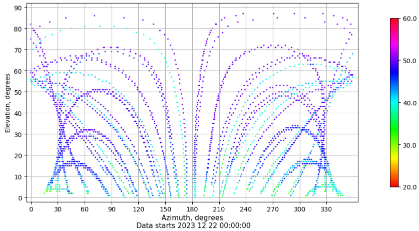
Azimuth-elevation plot for station ZFRA. Signal to Noise S1C Data file ZFRA00ESP_R_2023356.xtr
