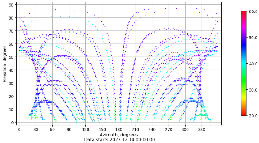
Azimuth-elevation plot for station ZFRA. Signal to Noise S1C Data file ZFRA00ESP_R_2023348.xtr
