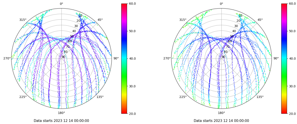
Skyplot for station ZFRA. Signal to Noise S1C Data file ZFRA00ESP_R_2023348.xtr Skyplot for station ZFRA. Signal to Noise S2P Data file ZFRA00ESP_R_2023348.xtr
