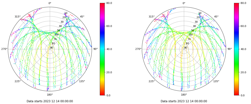
Skyplot for station ZFRA. Parameter M1C Data file ZFRA00ESP_R_2023348.xtr Skyplot for station ZFRA. Parameter M2P Data file ZFRA00ESP_R_2023348.xtr
