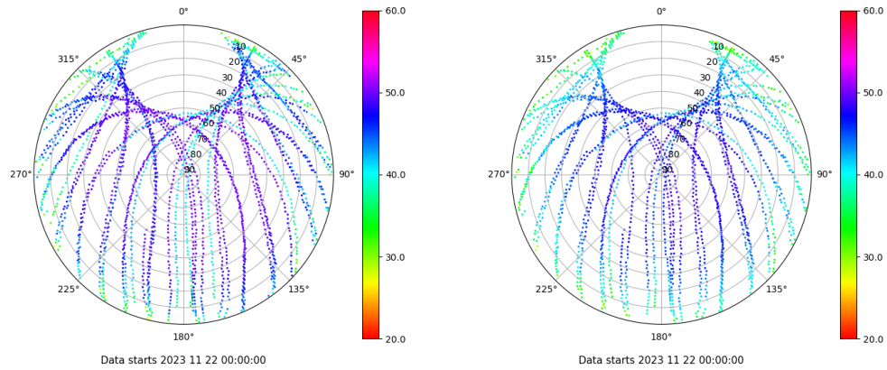
Skyplot for station ZFRA. Signal to Noise S1C Data file ZFRA00ESP_R_2023326.xtr Skyplot for station ZFRA. Signal to Noise S2P Data file ZFRA00ESP_R_2023326.xtr
