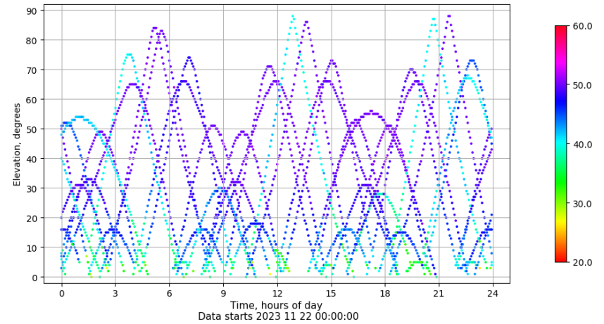
Time-elevation plot for station ZFRA. Signal to Noise S1C Data file ZFRA00ESP_R_2023326.xtr
