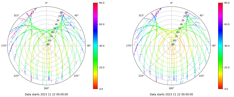
Skyplot for station ZFRA. Parameter M1C Data file ZFRA00ESP_R_2023326.xtr Skyplot for station ZFRA. Parameter M2P Data file ZFRA00ESP_R_2023326.xtr
