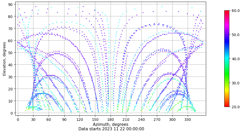
Azimuth-elevation plot for station ZFRA. Signal to Noise S1C Data file ZFRA00ESP_R_2023326.xtr
