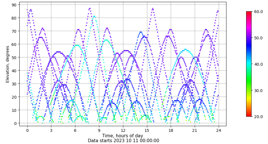
Time-elevation plot for station ZFRA. Signal to Noise S1C Data file ZFRA00ESP_R_2023284.xtr
