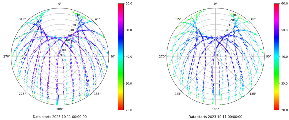
Skyplot for station ZFRA. Signal to Noise S1C Data file ZFRA00ESP_R_2023284.xtr Skyplot for station ZFRA. Signal to Noise S2P Data file ZFRA00ESP_R_2023284.xtr
