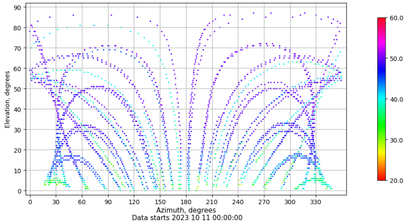
Azimuth-elevation plot for station ZFRA. Signal to Noise S1C Data file ZFRA00ESP_R_2023284.xtr
