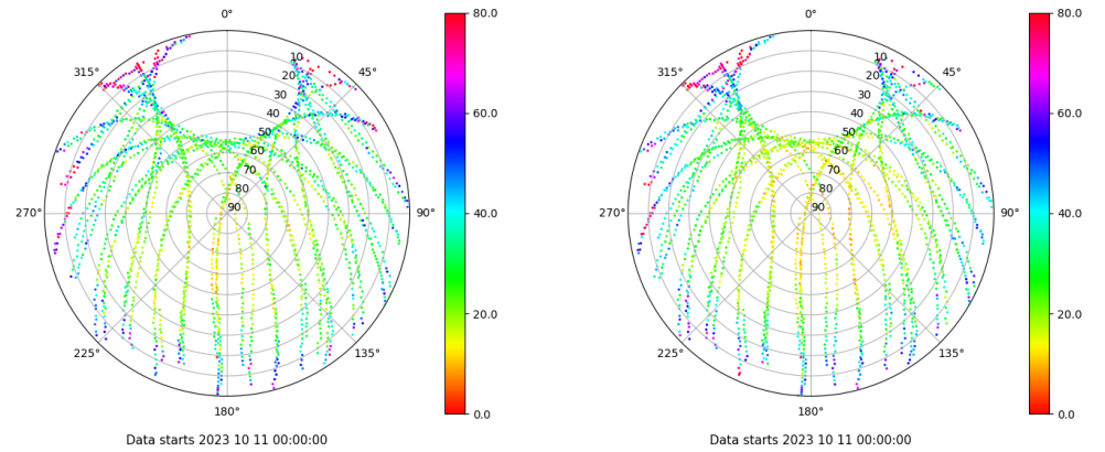
Skyplot for station ZFRA. Parameter M1C Data file ZFRA00ESP_R_2023284.xtr Skyplot for station ZFRA. Parameter M2P Data file ZFRA00ESP_R_2023284.xtr
