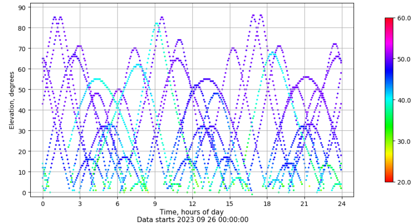
Time-elevation plot for station ZFRA. Signal to Noise S1C Data file ZFRA00ESP_R_2023269.xtr
