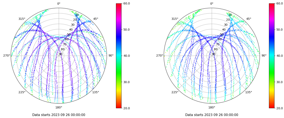
Skyplot for station ZFRA. Signal to Noise S1C Data file ZFRA00ESP_R_2023269.xtr Skyplot for station ZFRA. Signal to Noise S2P Data file ZFRA00ESP_R_2023269.xtr
