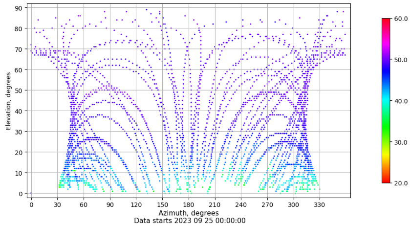
Azimuth-elevation plot for station ZFRA. Signal to Noise S1C Data file ZFRA00ESP_R_2023268.xtr
