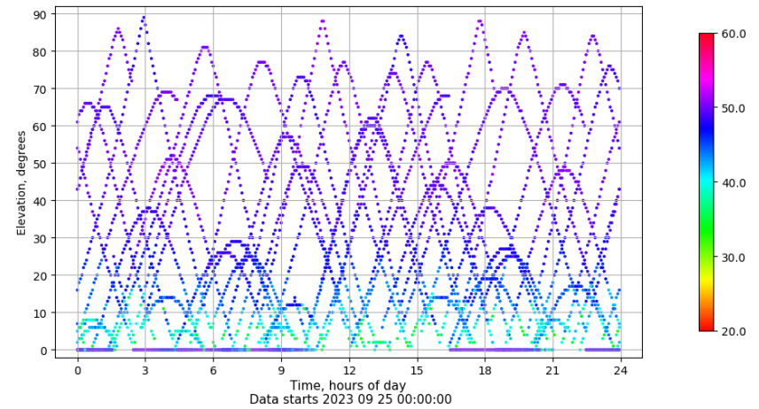
Time-elevation plot for station ZFRA. Signal to Noise S1C Data file ZFRA00ESP_R_2023268.xtr
