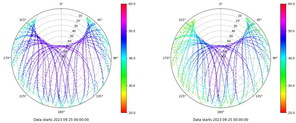
Skyplot for station ZFRA. Signal to Noise S1C Data file ZFRA00ESP_R_2023268.xtr Skyplot for station ZFRA. Signal to Noise S2W Data file ZFRA00ESP_R_2023268.xtr
