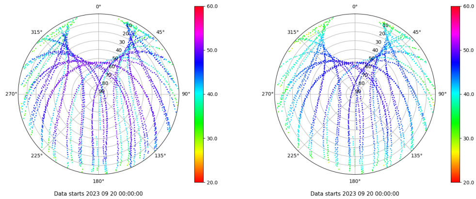
Skyplot for station ZFRA. Signal to Noise S1C Data file ZFRA00ESP_R_2023263.xtr Skyplot for station ZFRA. Signal to Noise S2P Data file ZFRA00ESP_R_2023263.xtr
