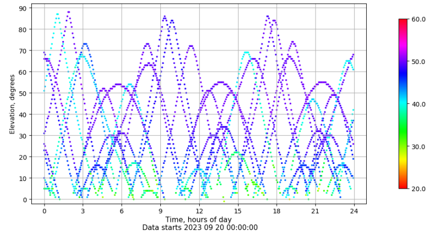
Time-elevation plot for station ZFRA. Signal to Noise S1C Data file ZFRA00ESP_R_2023263.xtr
