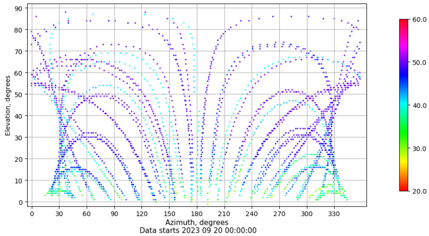
Azimuth-elevation plot for station ZFRA. Signal to Noise S1C Data file ZFRA00ESP_R_2023263.xtr
