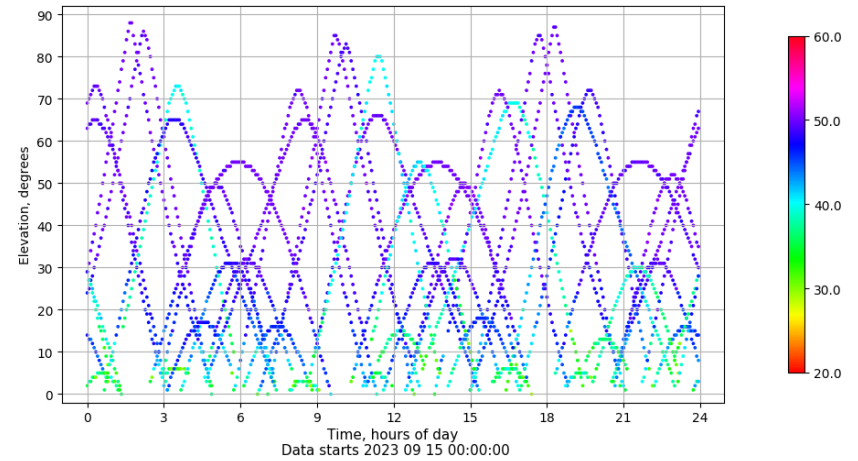
Time-elevation plot for station ZFRA. Signal to Noise S1C Data file ZFRA00ESP_R_2023258.xtr
