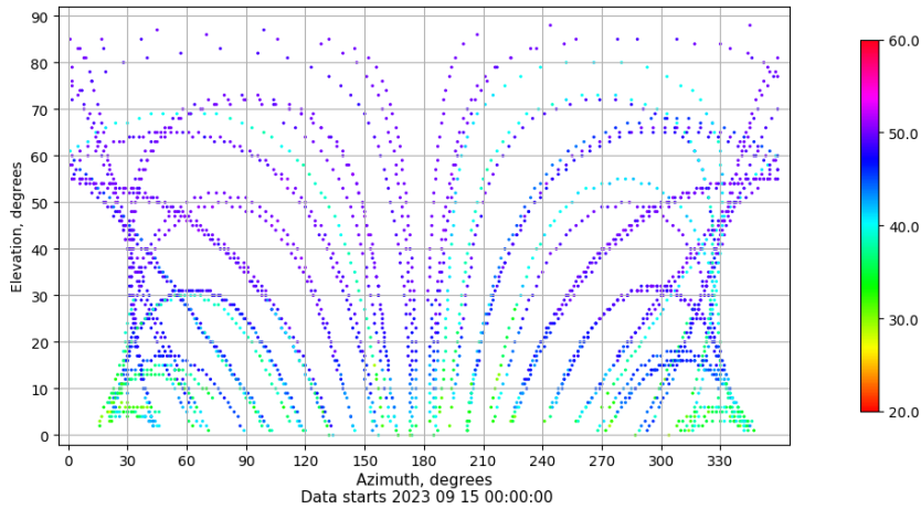
Azimuth-elevation plot for station ZFRA. Signal to Noise S1C Data file ZFRA00ESP_R_2023258.xtr
