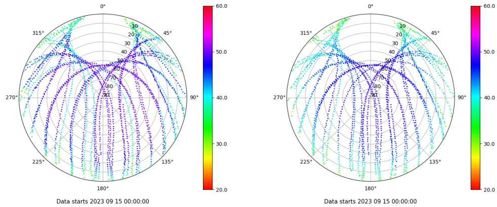
Skyplot for station ZFRA. Signal to Noise S1C Data file ZFRA00ESP_R_2023258.xtr Skyplot for station ZFRA. Signal to Noise S2P Data file ZFRA00ESP_R_2023258.xtr
