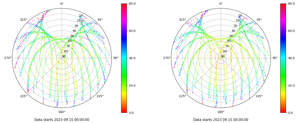
Skyplot for station ZFRA. Parameter M1C Data file ZFRA00ESP_R_2023258.xtr Skyplot for station ZFRA. Parameter M2P Data file ZFRA00ESP_R_2023258.xtr
